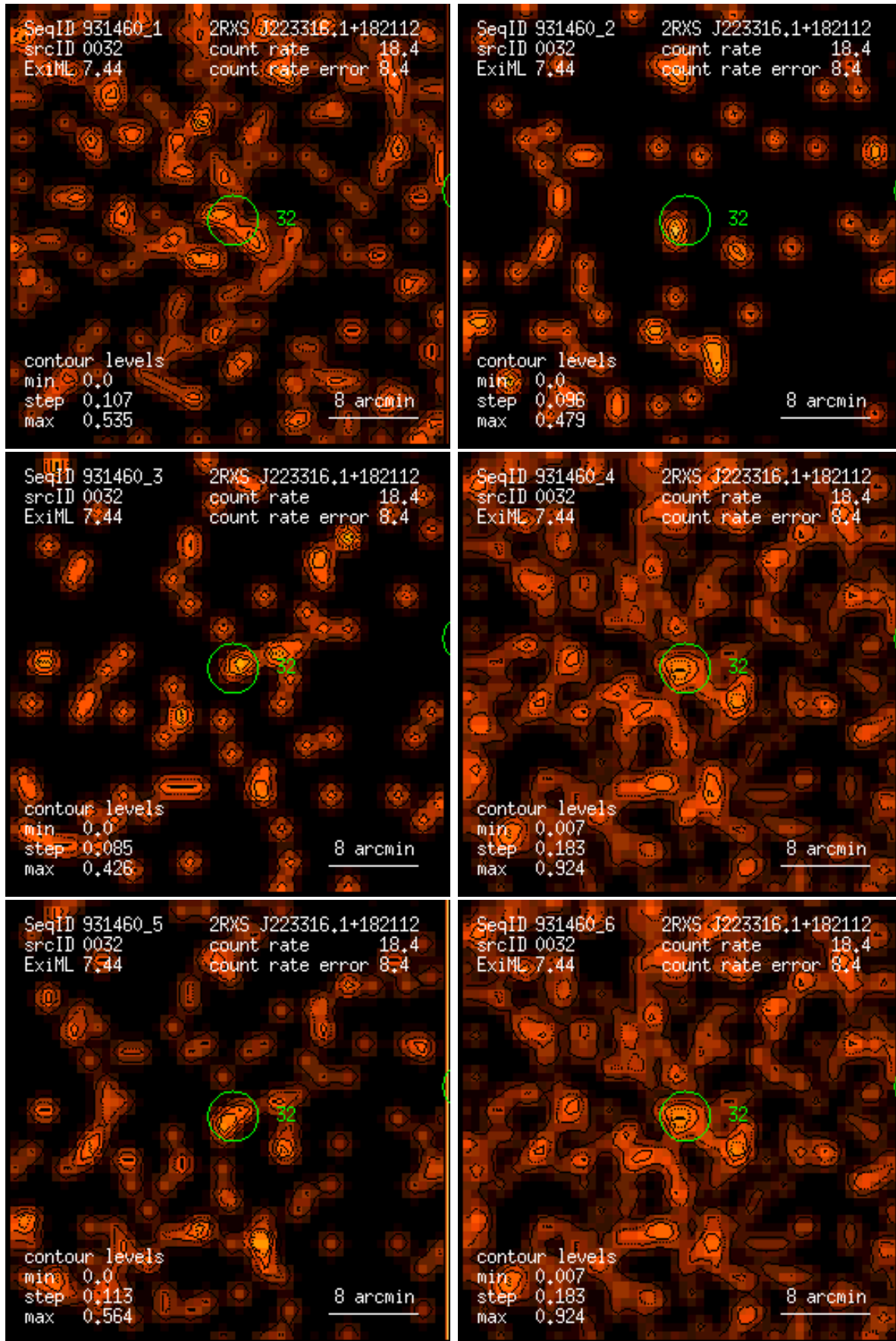
Figure 32: RASS 931460: detection 0032: band rate images, Gaussian filter: (1) PSPC channels 11 – 41, (2) 52 – 90, (3) 91 – 201, (4) 11 – 235, (5) 52 – 201, (6) 11 – 201. Broad band rates in counts/ks. Band rate contour levels in counts/ks/arcmin 2 .
