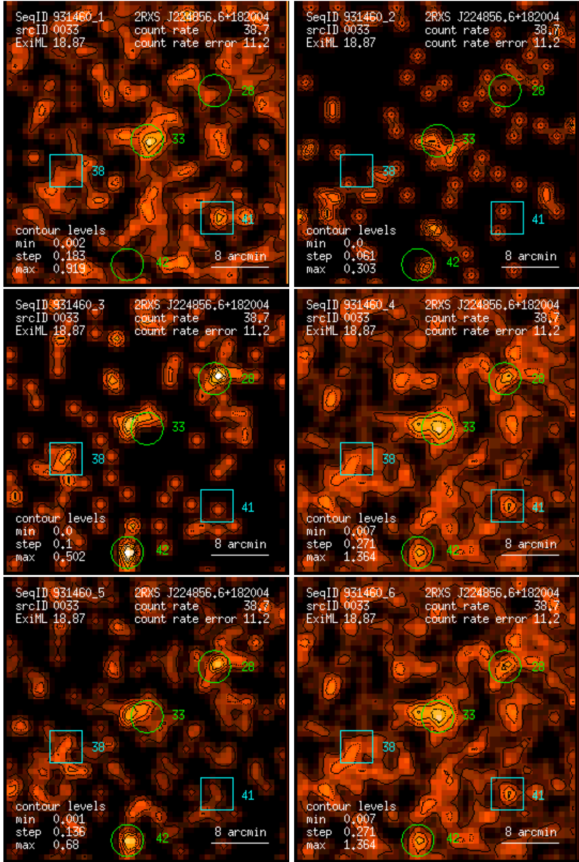
Figure 33: RASS 931460: detection 0033: band rate images, Gaussian filter: (1) PSPC channels 11 – 41, (2) 52 – 90, (3) 91 – 201, (4) 11 – 235, (5) 52 – 201, (6) 11 – 201. Broad band rates in counts/ks. Band rate contour levels in counts/ks/arcmin 2 .
