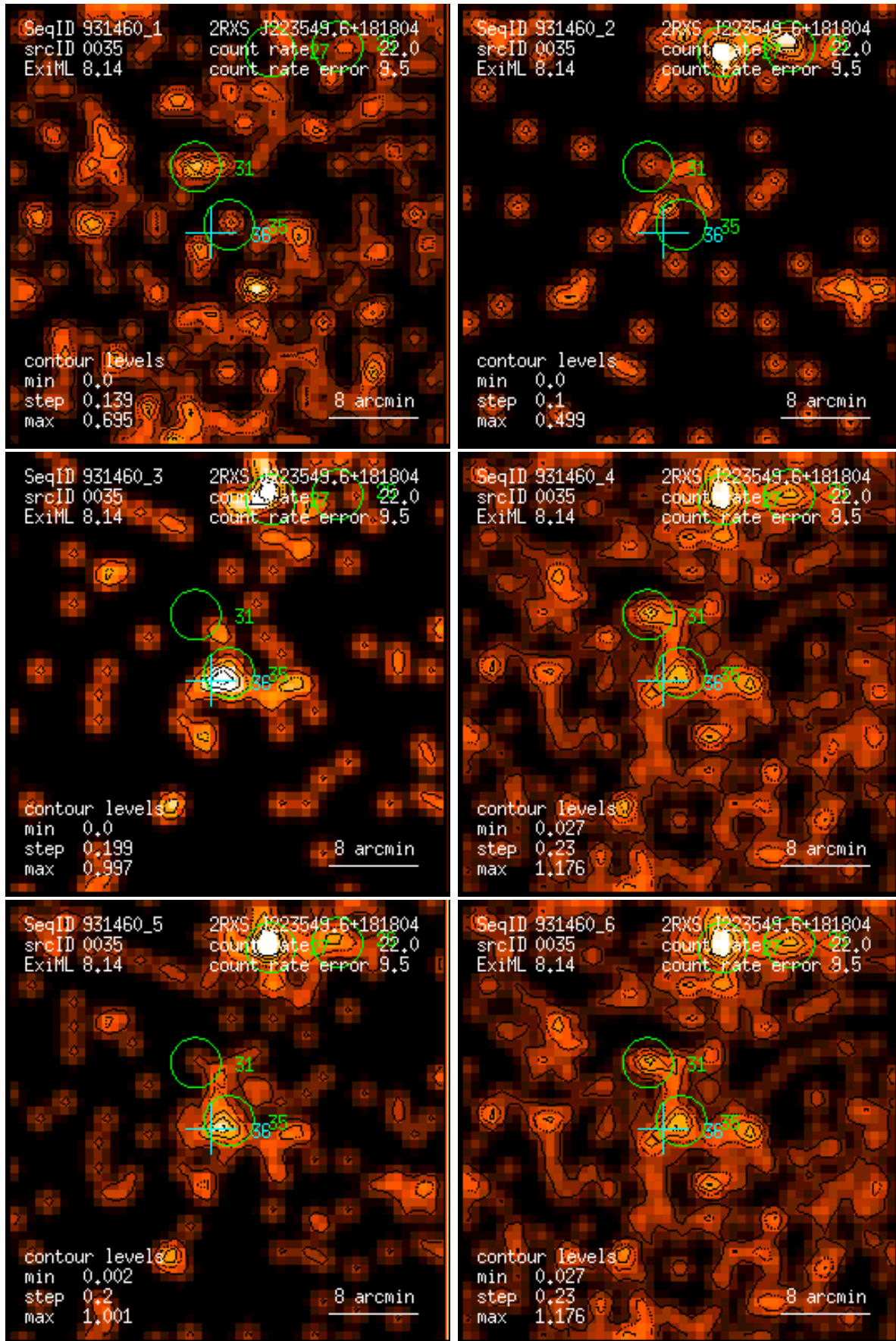
Figure 35: RASS 931460: detection 0035: band rate images, Gaussian filter: (1) PSPC channels 11 – 41, (2) 52 – 90, (3) 91 – 201, (4) 11 – 235, (5) 52 – 201, (6) 11 – 201. Broad band rates in counts/ks. Band rate contour levels in counts/ks/arcmin 2 .
