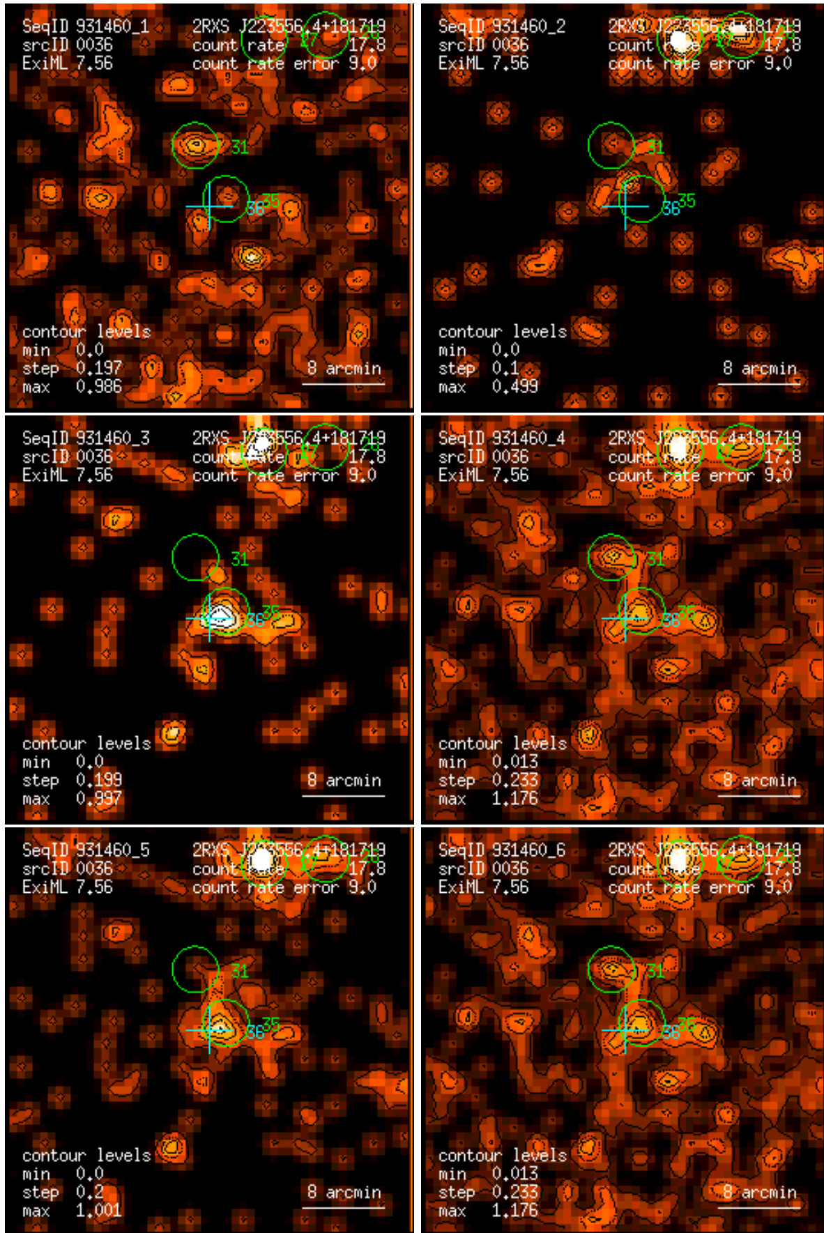
Figure 36: RASS 931460: detection 0036: band rate images, Gaussian filter: (1) PSPC channels 11 – 41, (2) 52 – 90, (3) 91 – 201, (4) 11 – 235, (5) 52 – 201, (6) 11 – 201. Broad band rates in counts/ks. Band rate contour levels in counts/ks/arcmin 2 .
