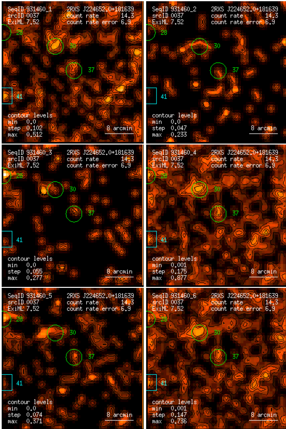
Figure 37: RASS 931460: detection 0037: band rate images, Gaussian filter: (1) PSPC channels 11 – 41, (2) 52 – 90, (3) 91 – 201, (4) 11 – 235, (5) 52 – 201, (6) 11 – 201. Broad band rates in counts/ks. Band rate contour levels in counts/ks/arcmin 2 .
