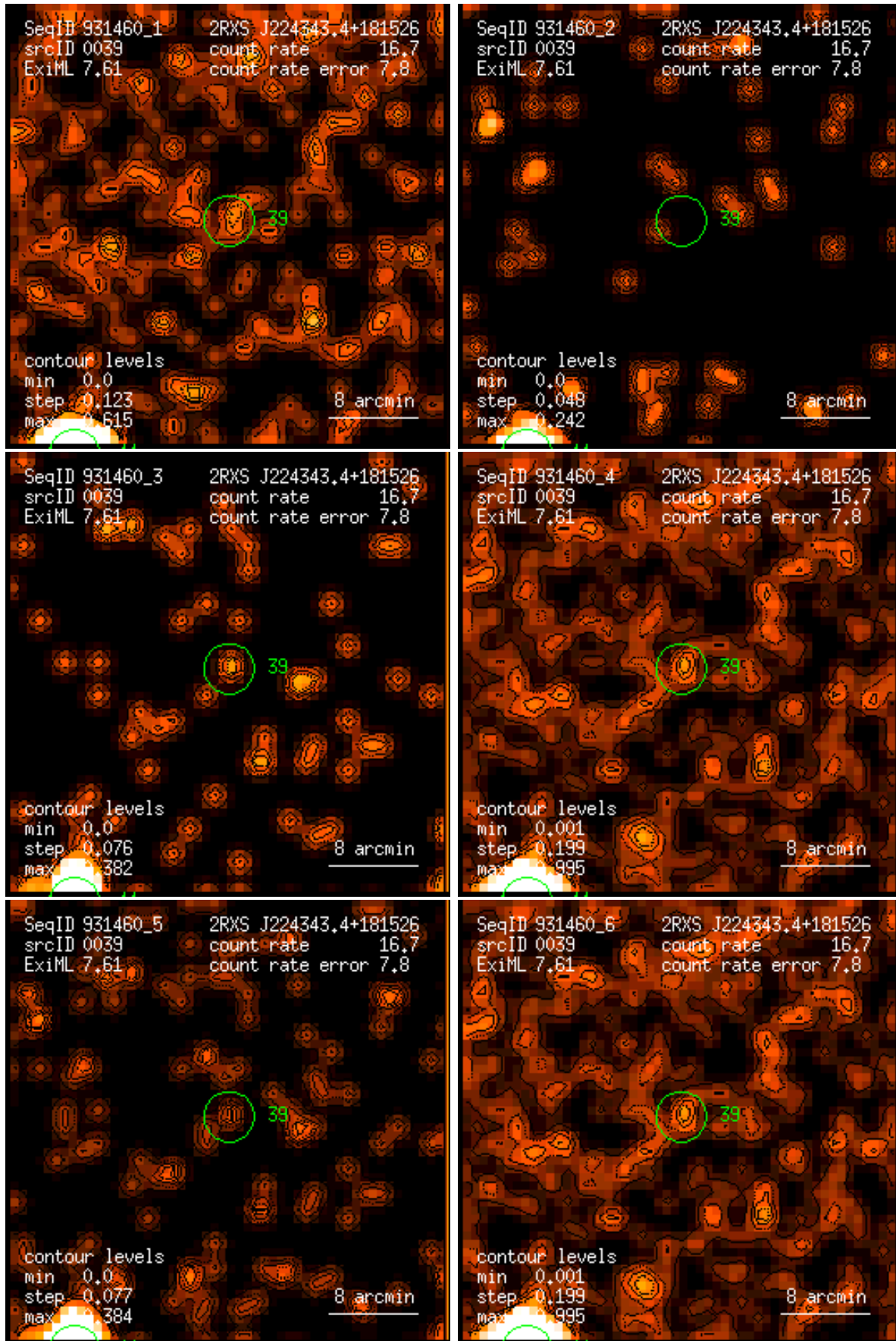
Figure 39: RASS 931460: detection 0039: band rate images, Gaussian filter: (1) PSPC channels 11 – 41, (2) 52 – 90, (3) 91 – 201, (4) 11 – 235, (5) 52 – 201, (6) 11 – 201. Broad band rates in counts/ks. Band rate contour levels in counts/ks/arcmin 2 .
