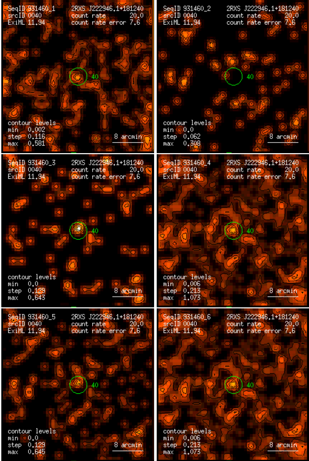
Figure 40: RASS 931460: detection 0040: band rate images, Gaussian filter: (1) PSPC channels 11 – 41, (2) 52 – 90, (3) 91 – 201, (4) 11 – 235, (5) 52 – 201, (6) 11 – 201. Broad band rates in counts/ks. Band rate contour levels in counts/ks/arcmin 2 .
