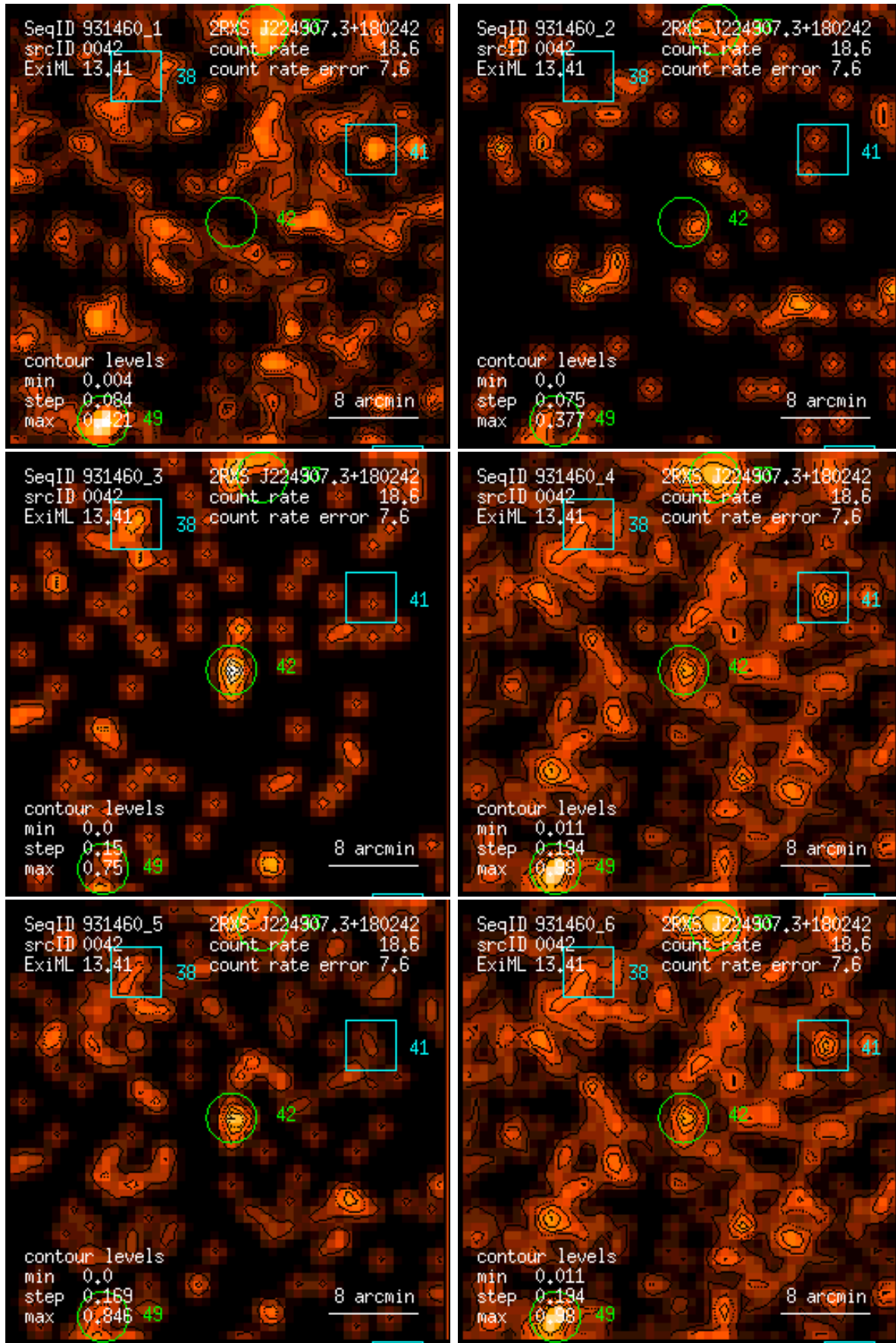
Figure 42: RASS 931460: detection 0042: band rate images, Gaussian filter: (1) PSPC channels 11 – 41, (2) 52 – 90, (3) 91 – 201, (4) 11 – 235, (5) 52 – 201, (6) 11 – 201. Broad band rates in counts/ks. Band rate contour levels in counts/ks/arcmin 2 .
