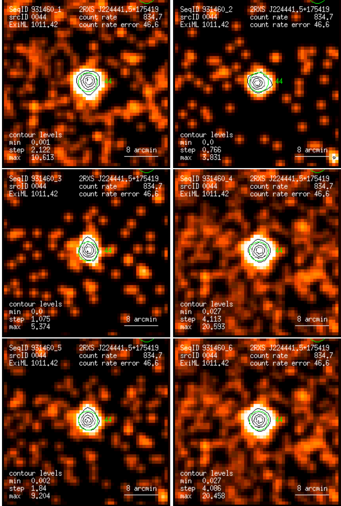
Figure 44: RASS 931460: detection 0044: band rate images, Gaussian filter: (1) PSPC channels 11 – 41, (2) 52 – 90, (3) 91 – 201, (4) 11 – 235, (5) 52 – 201, (6) 11 – 201. Broad band rates in counts/ks. Band rate contour levels in counts/ks/arcmin 2 .
