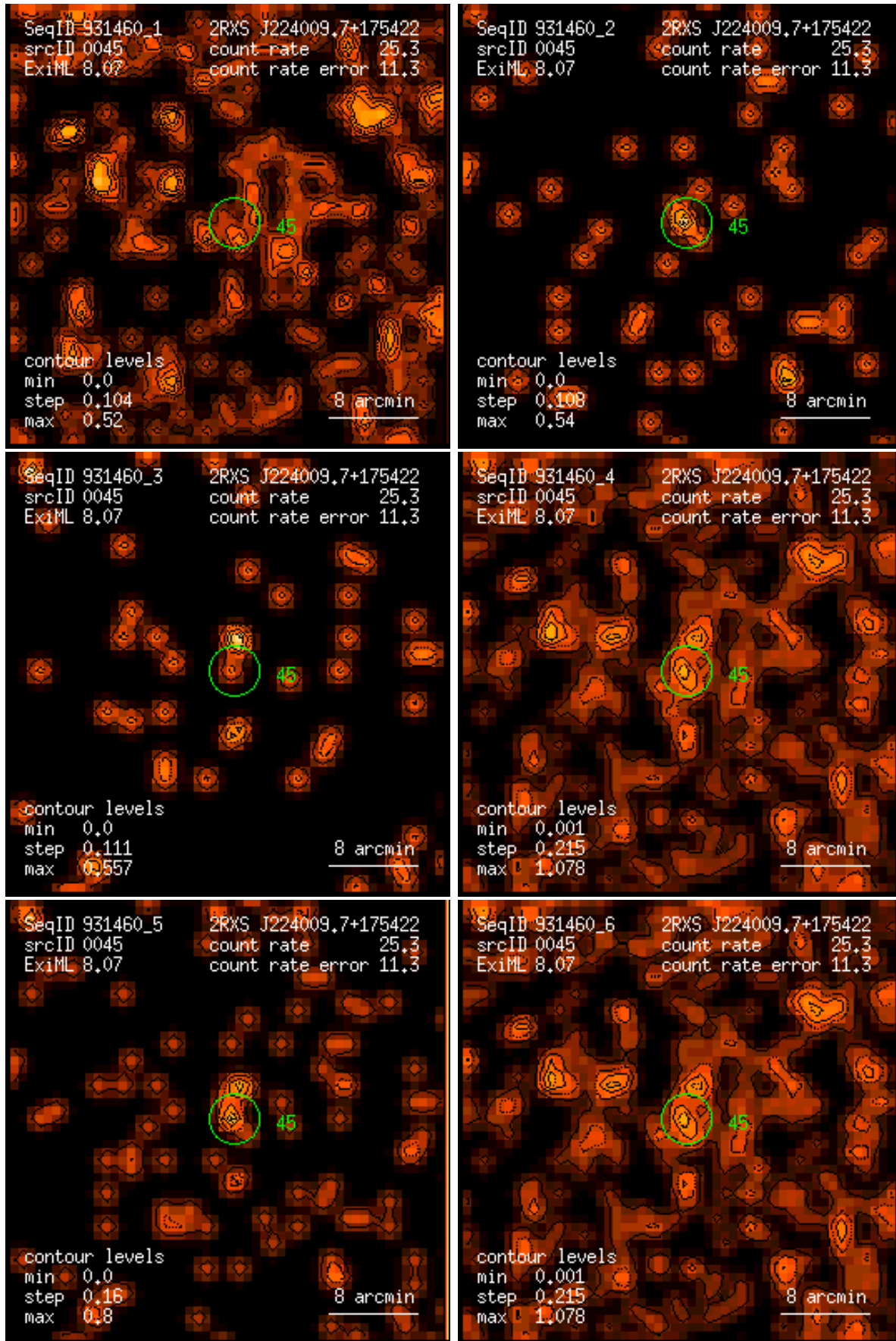
Figure 45: RASS 931460: detection 0045: band rate images, Gaussian filter: (1) PSPC channels 11 – 41, (2) 52 – 90, (3) 91 – 201, (4) 11 – 235, (5) 52 – 201, (6) 11 – 201. Broad band rates in counts/ks. Band rate contour levels in counts/ks/arcmin 2 .
