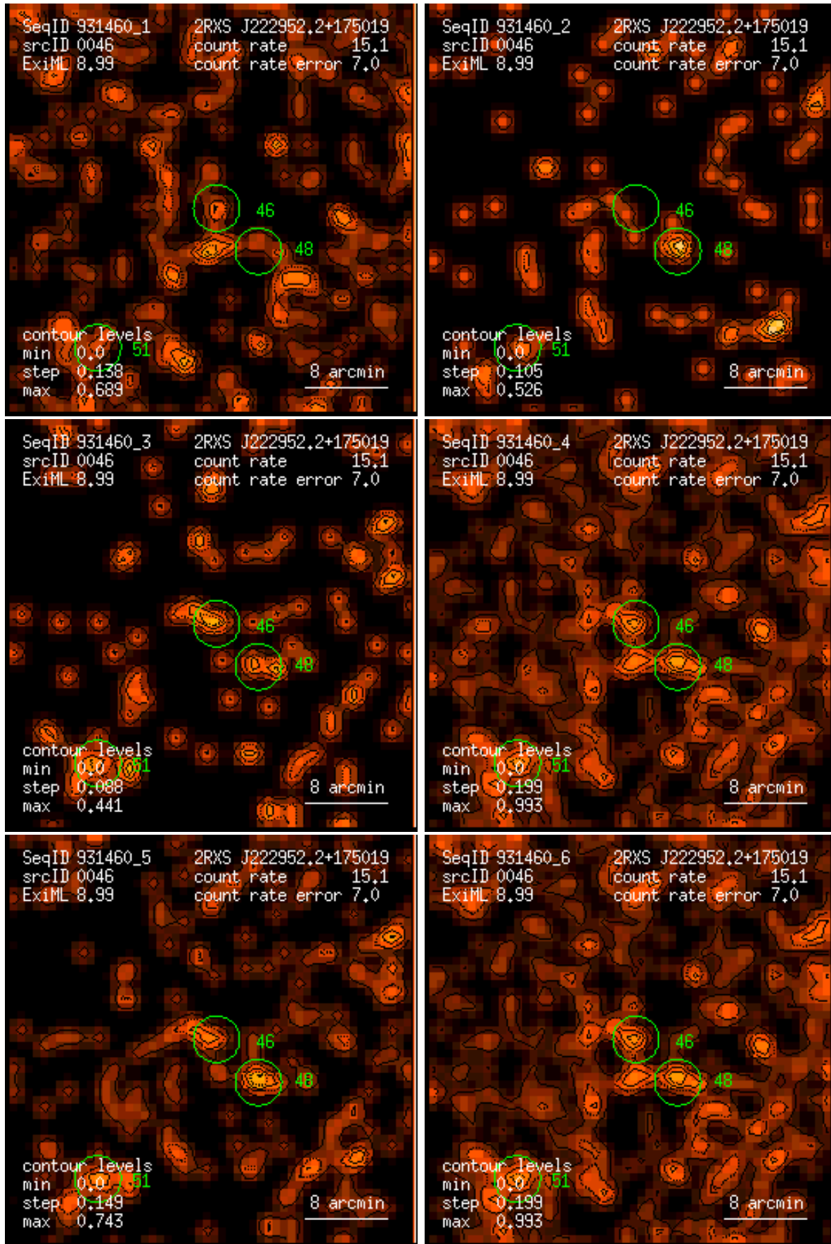
Figure 46: RASS 931460: detection 0046: band rate images, Gaussian filter: (1) PSPC channels 11 – 41, (2) 52 – 90, (3) 91 – 201, (4) 11 – 235, (5) 52 – 201, (6) 11 – 201. Broad band rates in counts/ks. Band rate contour levels in counts/ks/arcmin 2 .
