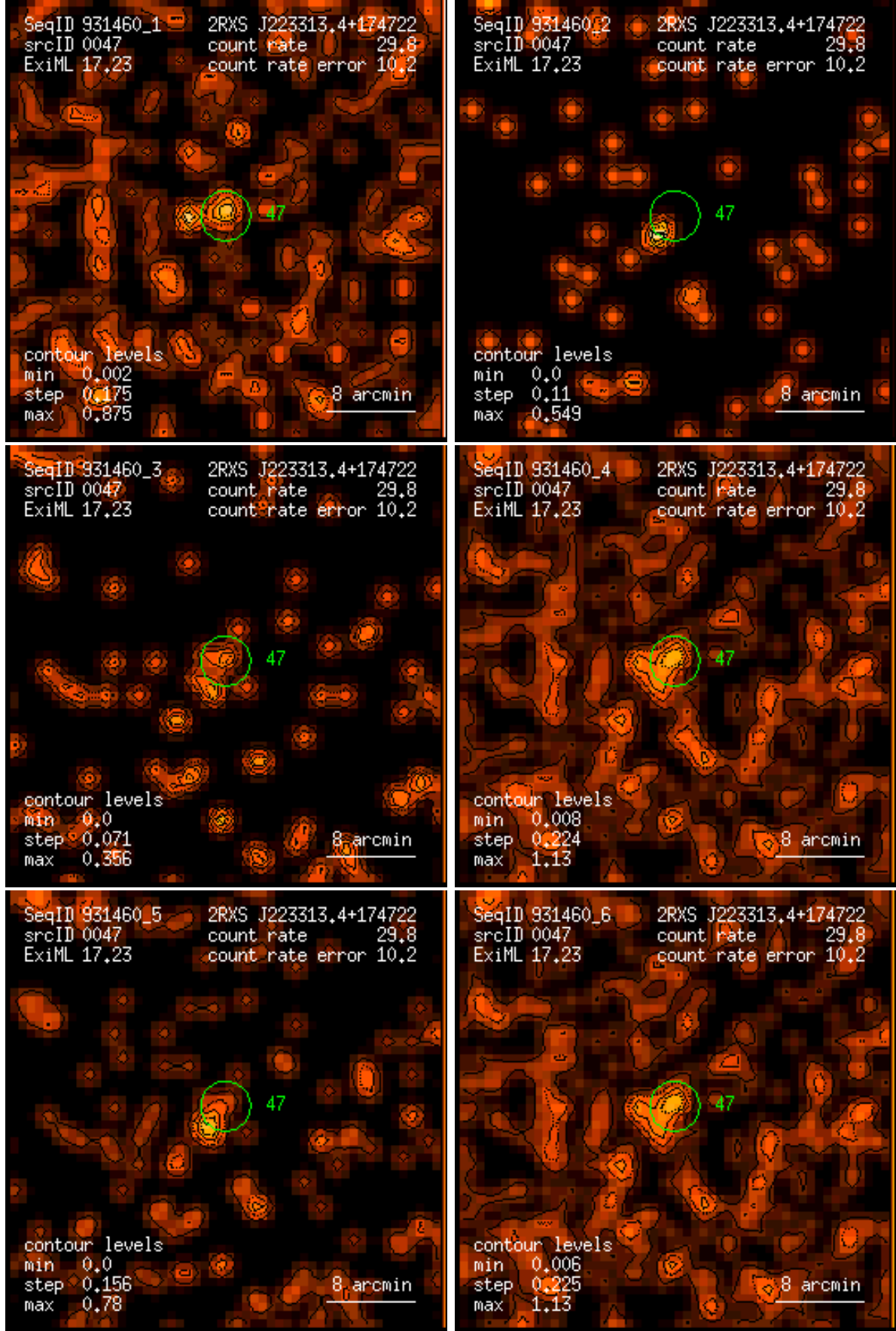
Figure 47: RASS 931460: detection 0047: band rate images, Gaussian filter: (1) PSPC channels 11 – 41, (2) 52 – 90, (3) 91 – 201, (4) 11 – 235, (5) 52 – 201, (6) 11 – 201. Broad band rates in counts/ks. Band rate contour levels in counts/ks/arcmin 2 .
