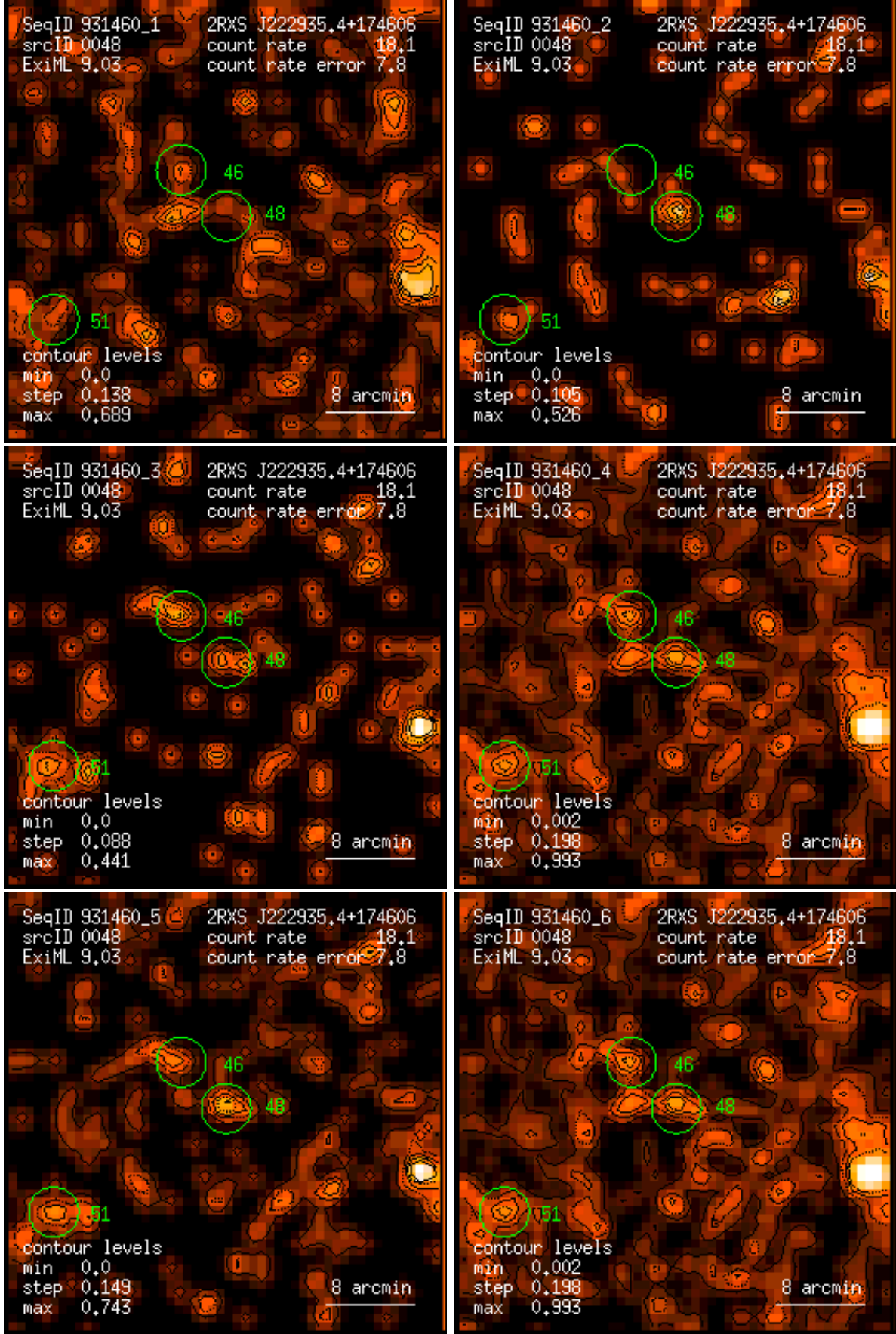
Figure 48: RASS 931460: detection 0048: band rate images, Gaussian filter: (1) PSPC channels 11 – 41, (2) 52 – 90, (3) 91 – 201, (4) 11 – 235, (5) 52 – 201, (6) 11 – 201. Broad band rates in counts/ks. Band rate contour levels in counts/ks/arcmin 2 .
