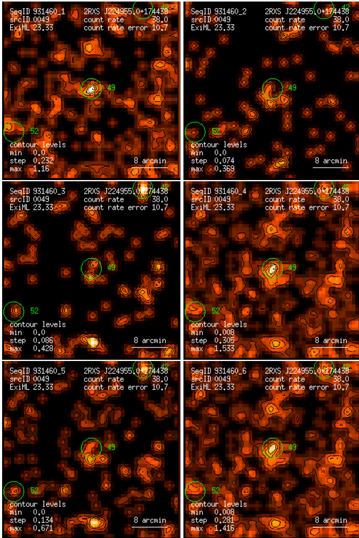
Figure 49: RASS 931460: detection 0049: band rate images, Gaussian filter: (1) PSPC channels 11 – 41, (2) 52 – 90, (3) 91 – 201, (4) 11 – 235, (5) 52 – 201, (6) 11 – 201. Broad band rates in counts/ks. Band rate contour levels in counts/ks/arcmin 2 .
