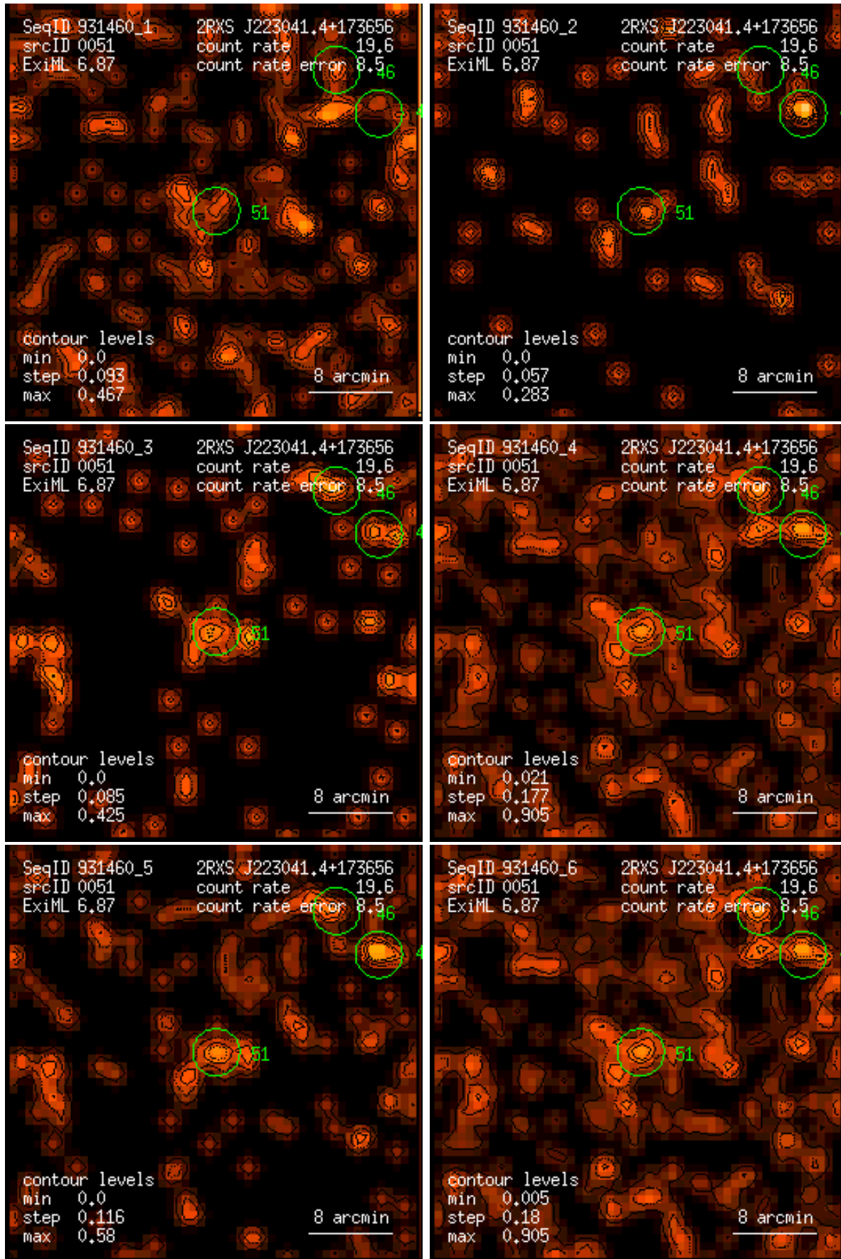
Figure 51: RASS 931460: detection 0051: band rate images, Gaussian filter: (1) PSPC channels 11 – 41, (2) 52 – 90, (3) 91 – 201, (4) 11 – 235, (5) 52 – 201, (6) 11 – 201. Broad band rates in counts/ks. Band rate contour levels in counts/ks/arcmin 2 .
