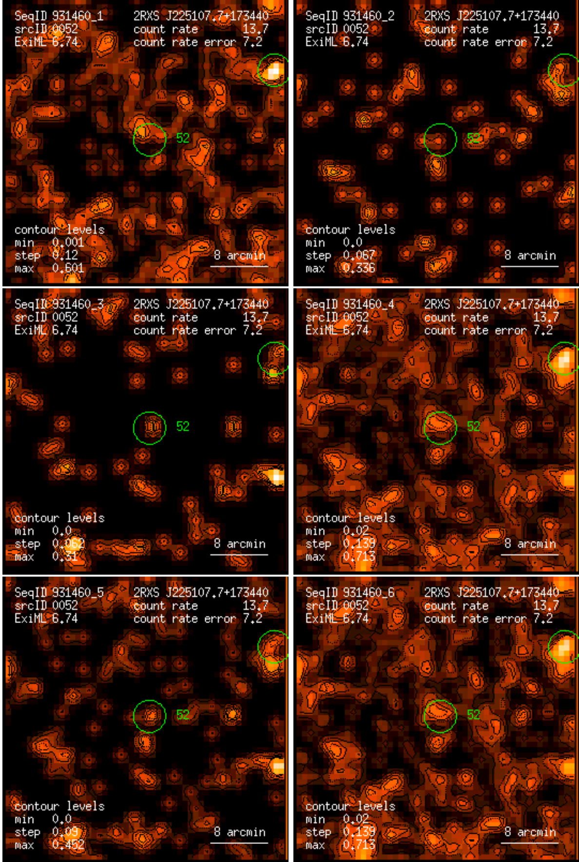
Figure 52: RASS 931460: detection 0052: band rate images, Gaussian filter: (1) PSPC channels 11 – 41, (2) 52 – 90, (3) 91 – 201, (4) 11 – 235, (5) 52 – 201, (6) 11 – 201. Broad band rates in counts/ks. Band rate contour levels in counts/ks/arcmin 2 .
