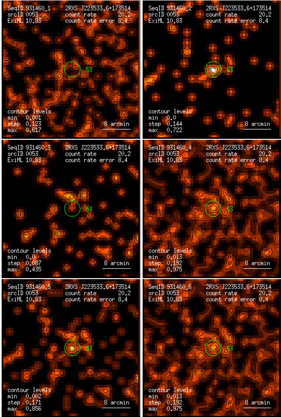
Figure 53: RASS 931460: detection 0053: band rate images, Gaussian filter: (1) PSPC channels 11 – 41, (2) 52 – 90, (3) 91 – 201, (4) 11 – 235, (5) 52 – 201, (6) 11 – 201. Broad band rates in counts/ks. Band rate contour levels in counts/ks/arcmin 2 .
