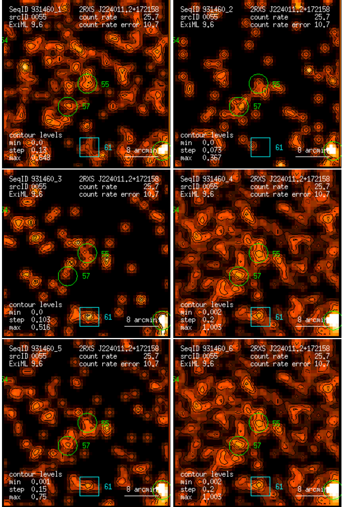
Figure 55: RASS 931460: detection 0055: band rate images, Gaussian filter: (1) PSPC channels 11 – 41, (2) 52 – 90, (3) 91 – 201, (4) 11 – 235, (5) 52 – 201, (6) 11 – 201. Broad band rates in counts/ks. Band rate contour levels in counts/ks/arcmin 2 .
