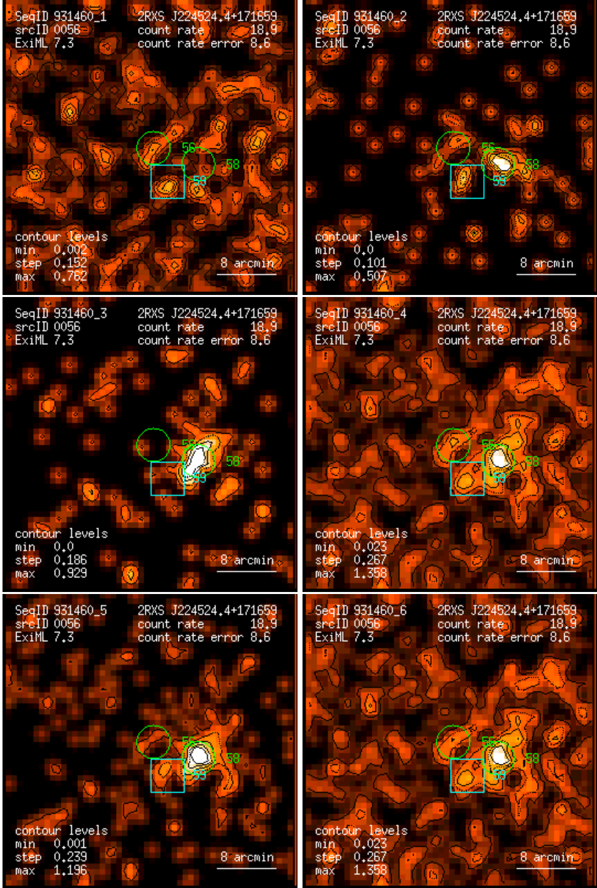
Figure 56: RASS 931460: detection 0056: band rate images, Gaussian filter: (1) PSPC channels 11 – 41, (2) 52 – 90, (3) 91 – 201, (4) 11 – 235, (5) 52 – 201, (6) 11 – 201. Broad band rates in counts/ks. Band rate contour levels in counts/ks/arcmin 2 .
