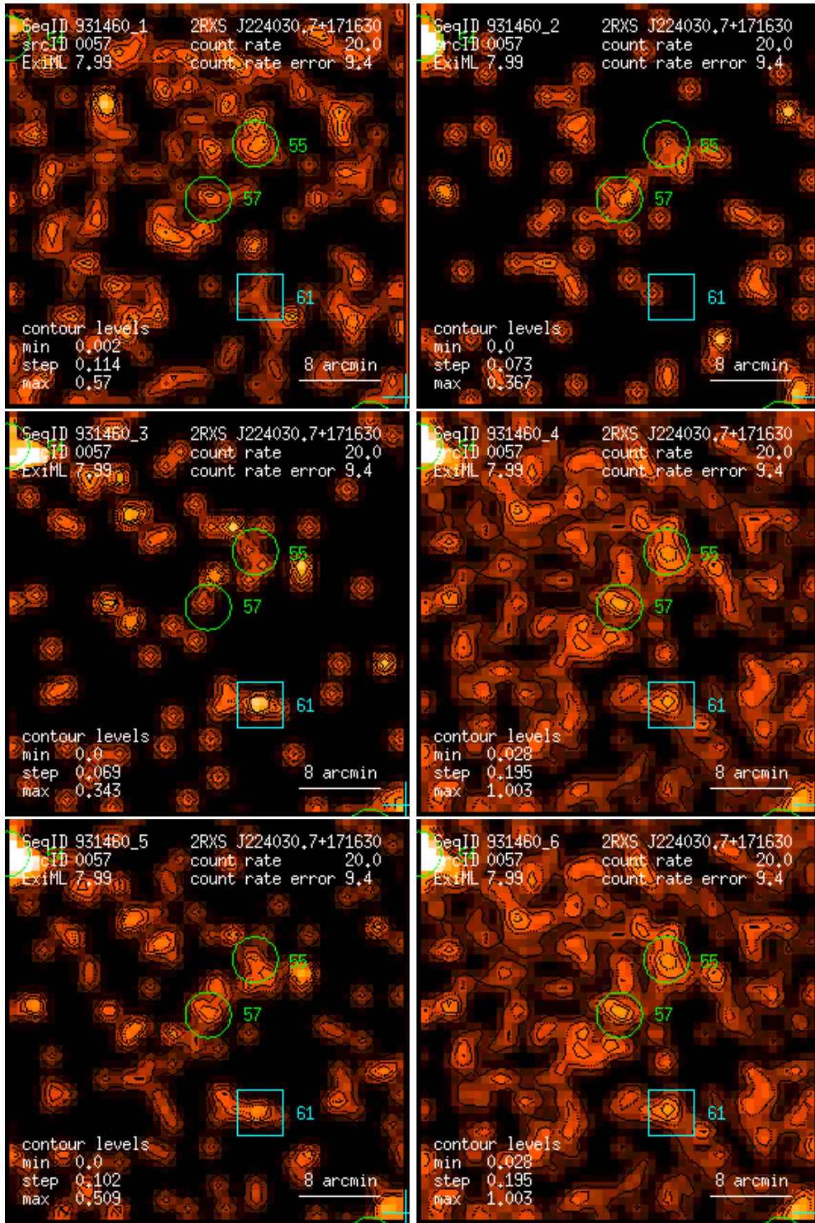
Figure 57: RASS 931460: detection 0057: band rate images, Gaussian filter: (1) PSPC channels 11 – 41, (2) 52 – 90, (3) 91 – 201, (4) 11 – 235, (5) 52 – 201, (6) 11 – 201. Broad band rates in counts/ks. Band rate contour levels in counts/ks/arcmin 2 .
