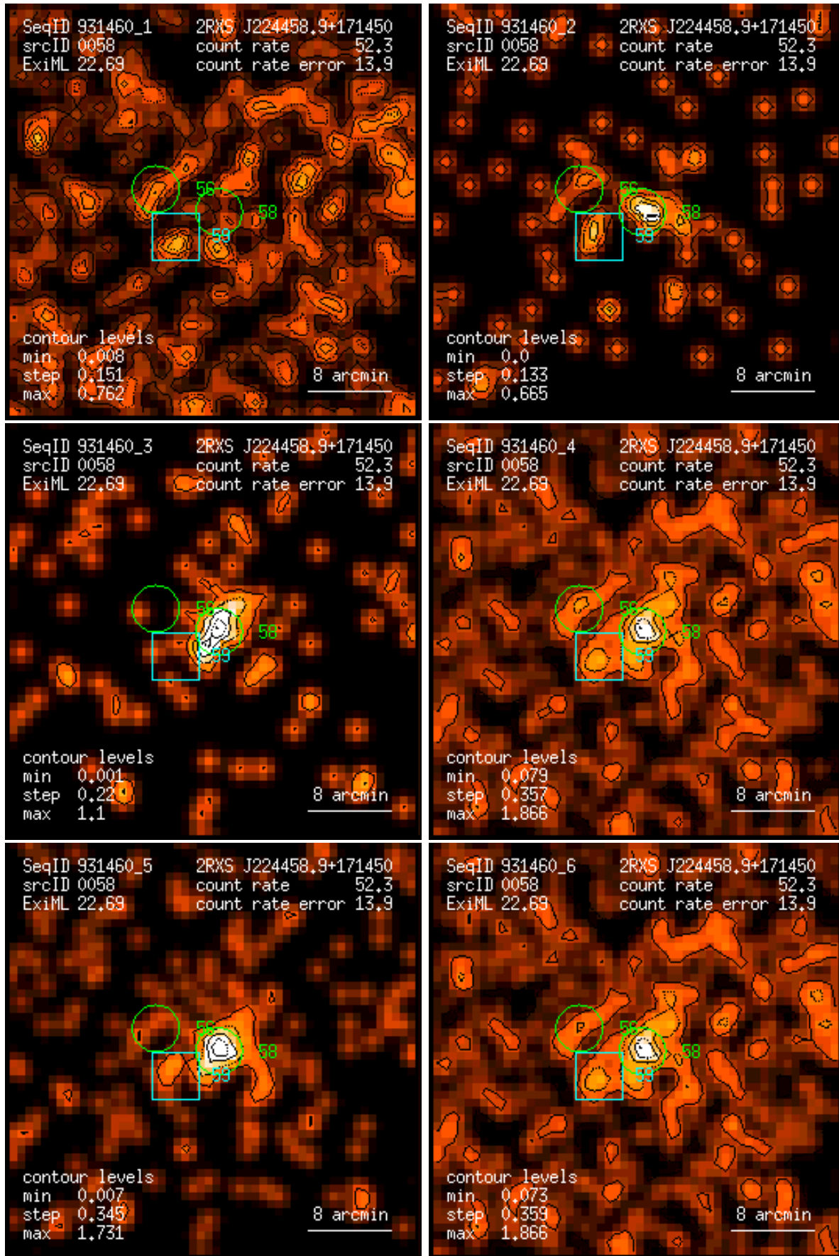
Figure 58: RASS 931460: detection 0058: band rate images, Gaussian filter: (1) PSPC channels 11 – 41, (2) 52 – 90, (3) 91 – 201, (4) 11 – 235, (5) 52 – 201, (6) 11 – 201. Broad band rates in counts/ks. Band rate contour levels in counts/ks/arcmin 2 .
