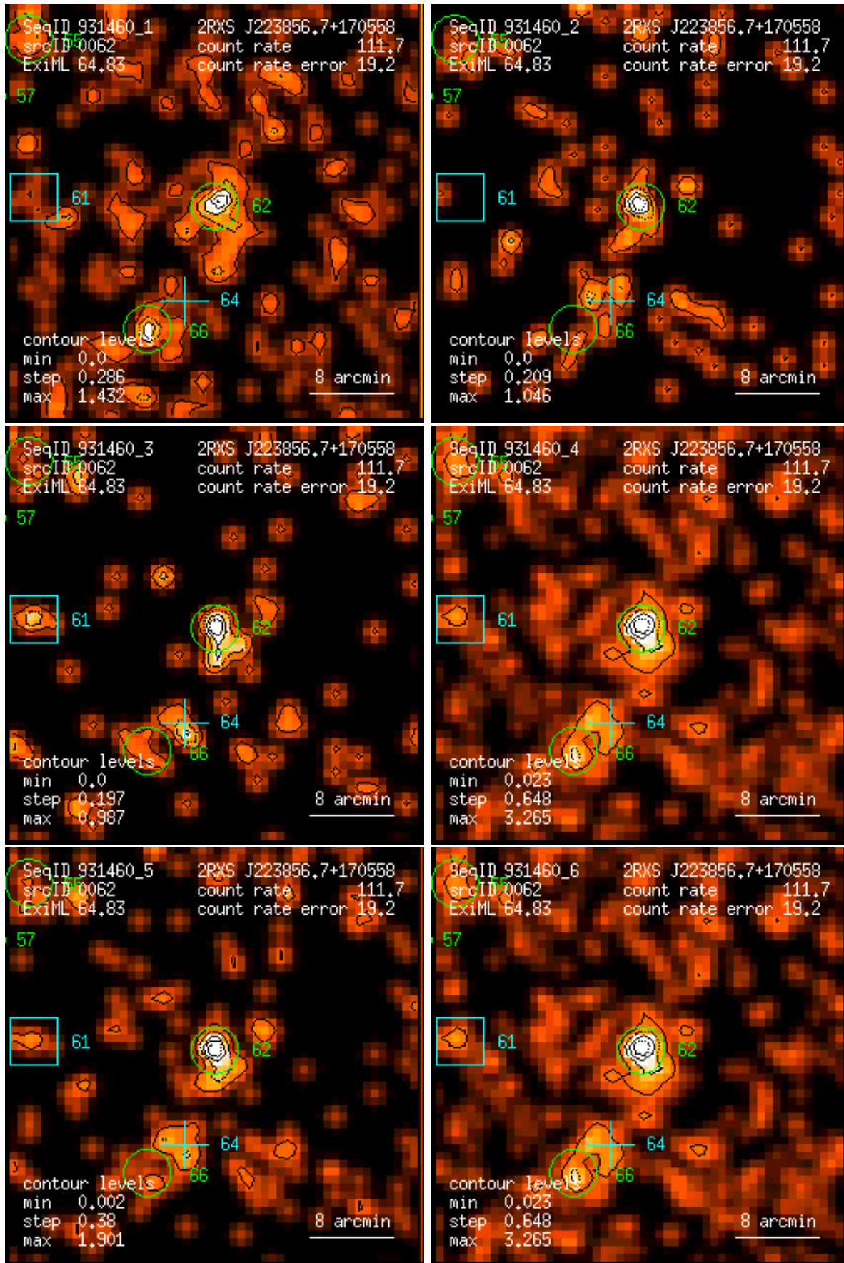
Figure 62: RASS 931460: detection 0062: band rate images, Gaussian filter: (1) PSPC channels 11 – 41, (2) 52 – 90, (3) 91 – 201, (4) 11 – 235, (5) 52 – 201, (6) 11 – 201. Broad band rates in counts/ks. Band rate contour levels in counts/ks/arcmin 2 .
