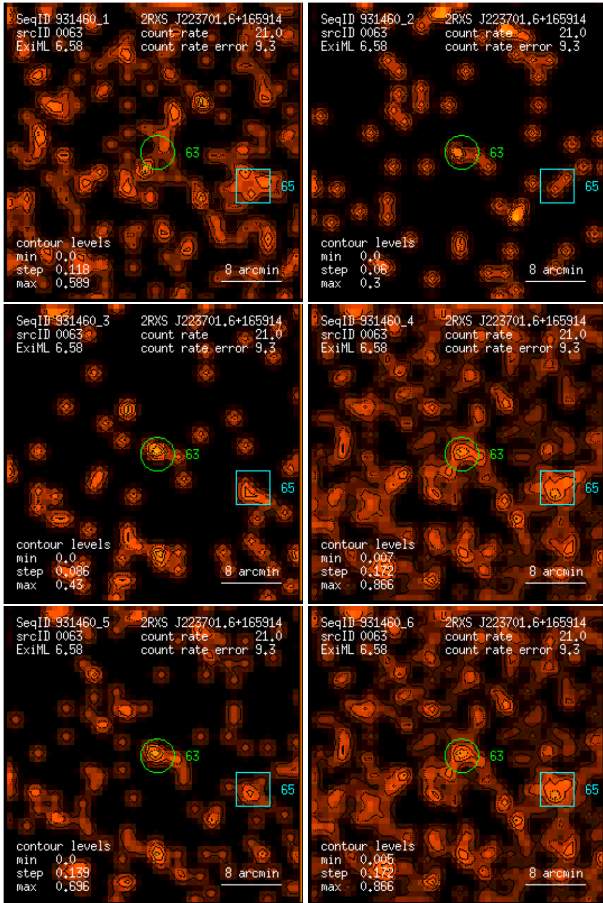
Figure 63: RASS 931460: detection 0063: band rate images, Gaussian filter: (1) PSPC channels 11 – 41, (2) 52 – 90, (3) 91 – 201, (4) 11 – 235, (5) 52 – 201, (6) 11 – 201. Broad band rates in counts/ks. Band rate contour levels in counts/ks/arcmin 2 .
