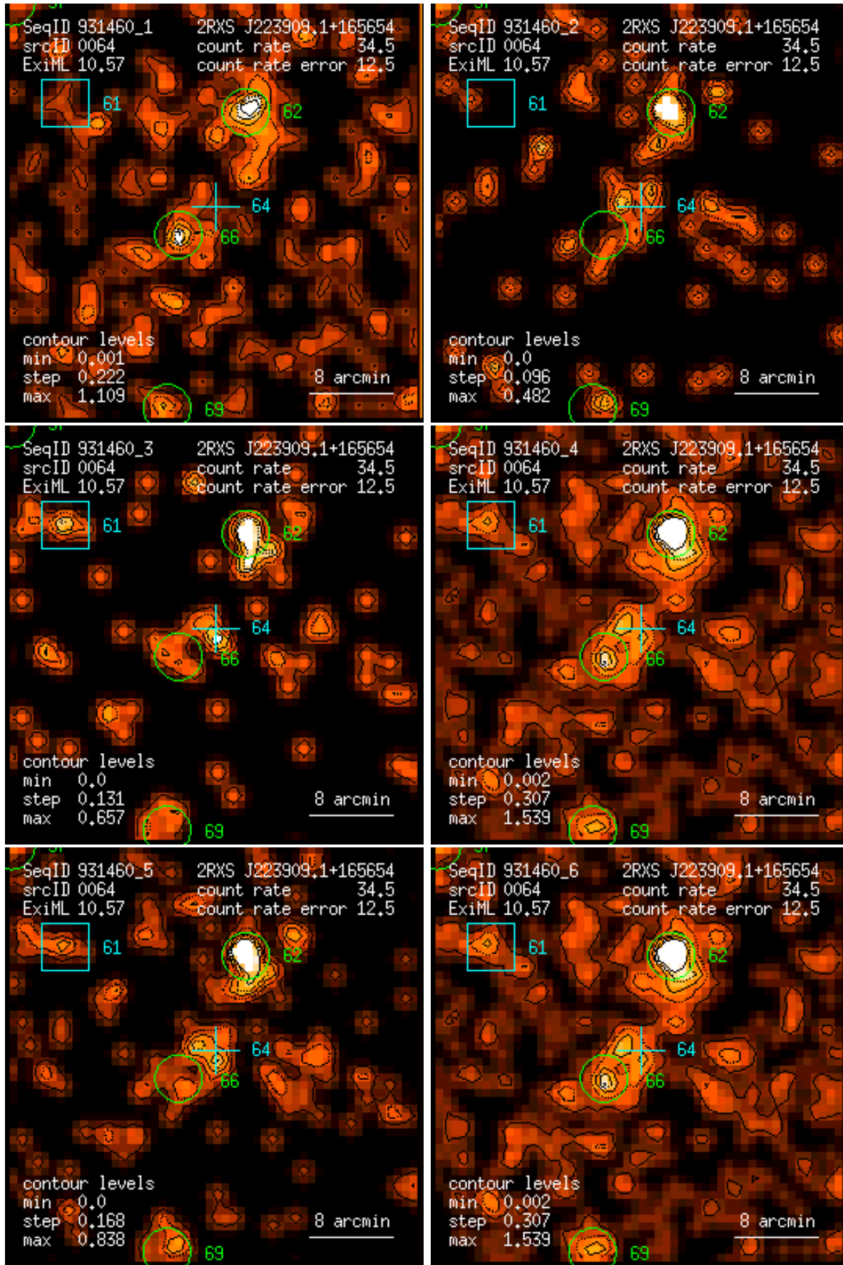
Figure 64: RASS 931460: detection 0064: band rate images, Gaussian filter: (1) PSPC channels 11 – 41, (2) 52 – 90, (3) 91 – 201, (4) 11 – 235, (5) 52 – 201, (6) 11 – 201. Broad band rates in counts/ks. Band rate contour levels in counts/ks/arcmin 2 .
