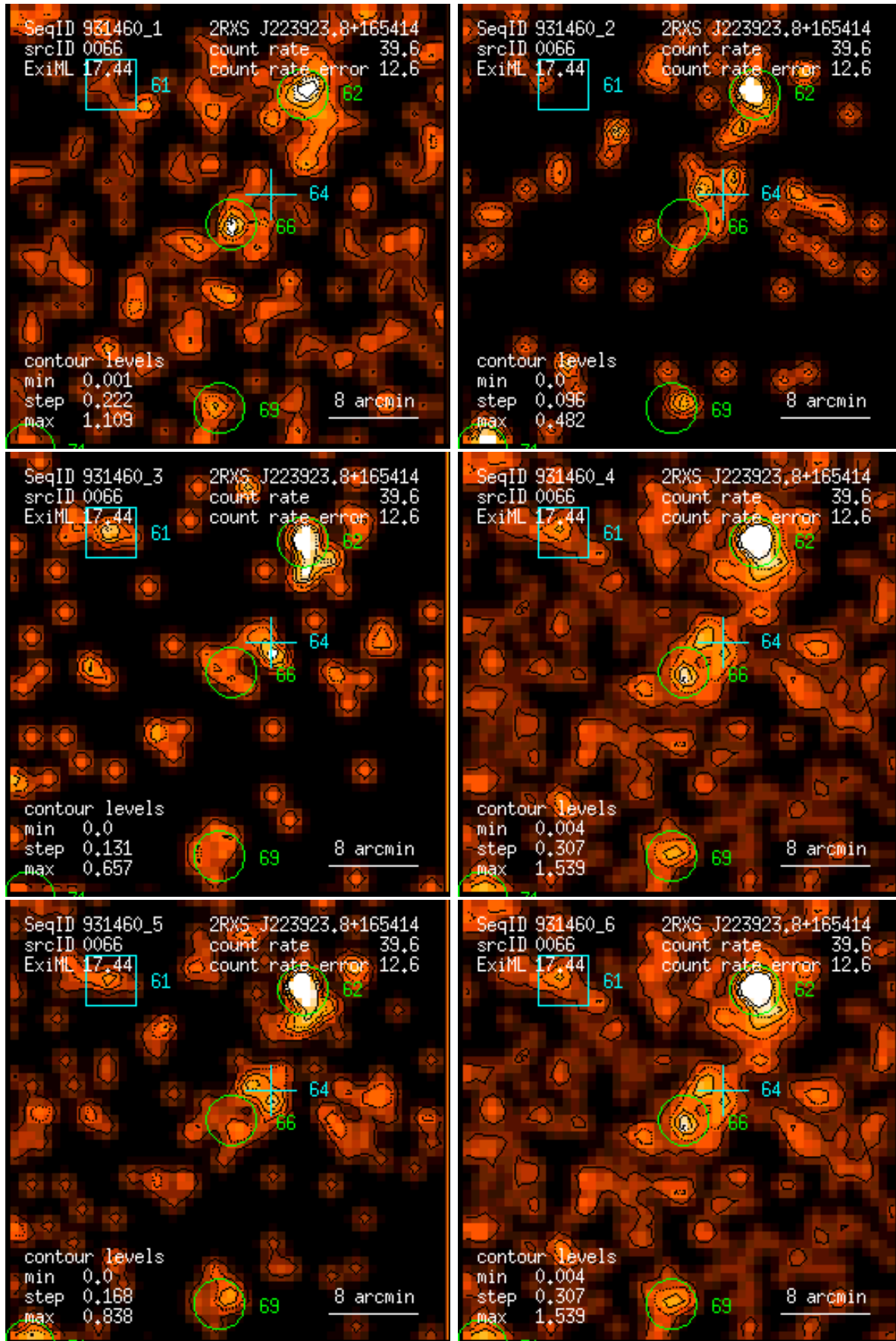
Figure 66: RASS 931460: detection 0066: band rate images, Gaussian filter: (1) PSPC channels 11 – 41, (2) 52 – 90, (3) 91 – 201, (4) 11 – 235, (5) 52 – 201, (6) 11 – 201. Broad band rates in counts/ks. Band rate contour levels in counts/ks/arcmin 2 .
