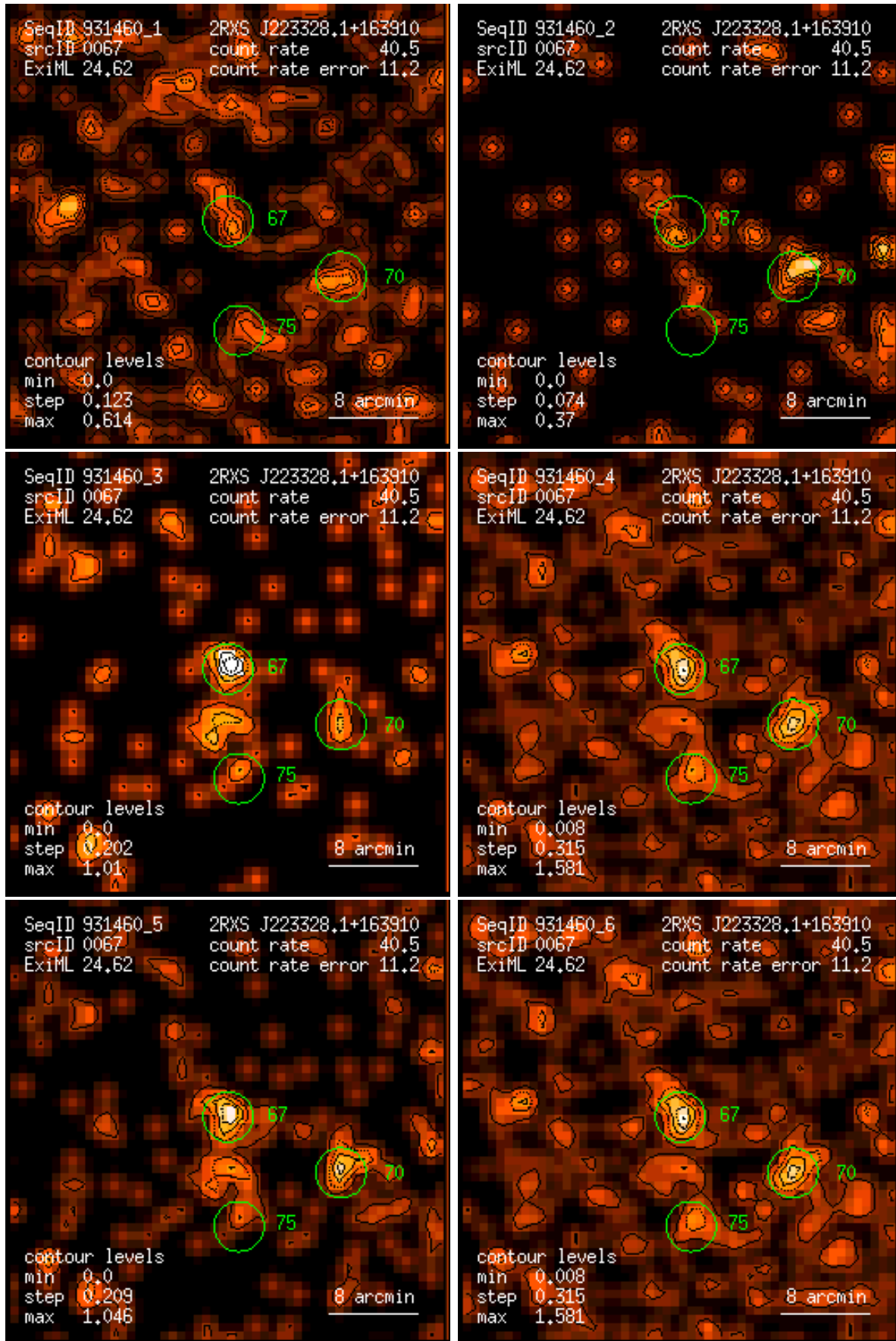
Figure 67: RASS 931460: detection 0067: band rate images, Gaussian filter: (1) PSPC channels 11 – 41, (2) 52 – 90, (3) 91 – 201, (4) 11 – 235, (5) 52 – 201, (6) 11 – 201. Broad band rates in counts/ks. Band rate contour levels in counts/ks/arcmin 2 .
