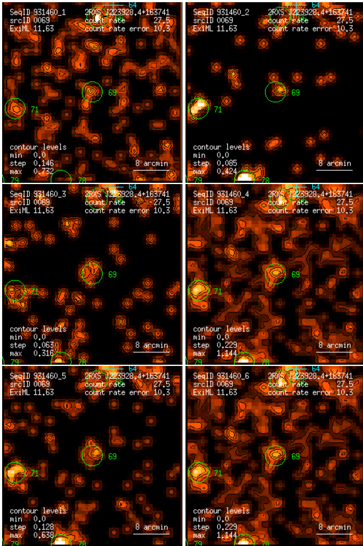
Figure 69: RASS 931460: detection 0069: band rate images, Gaussian filter: (1) PSPC channels 11 – 41, (2) 52 – 90, (3) 91 – 201, (4) 11 – 235, (5) 52 – 201, (6) 11 – 201. Broad band rates in counts/ks. Band rate contour levels in counts/ks/arcmin 2 .
