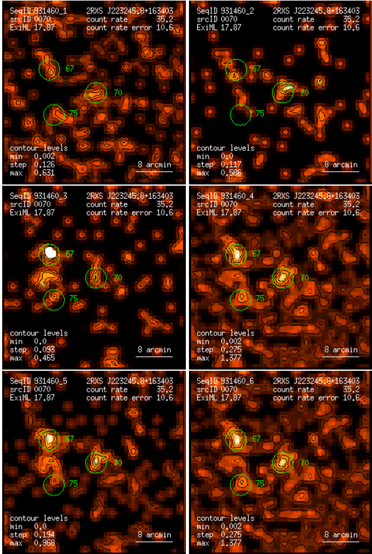
Figure 70: RASS 931460: detection 0070: band rate images, Gaussian filter: (1) PSPC channels 11 – 41, (2) 52 – 90, (3) 91 – 201, (4) 11 – 235, (5) 52 – 201, (6) 11 – 201. Broad band rates in counts/ks. Band rate contour levels in counts/ks/arcmin 2 .
