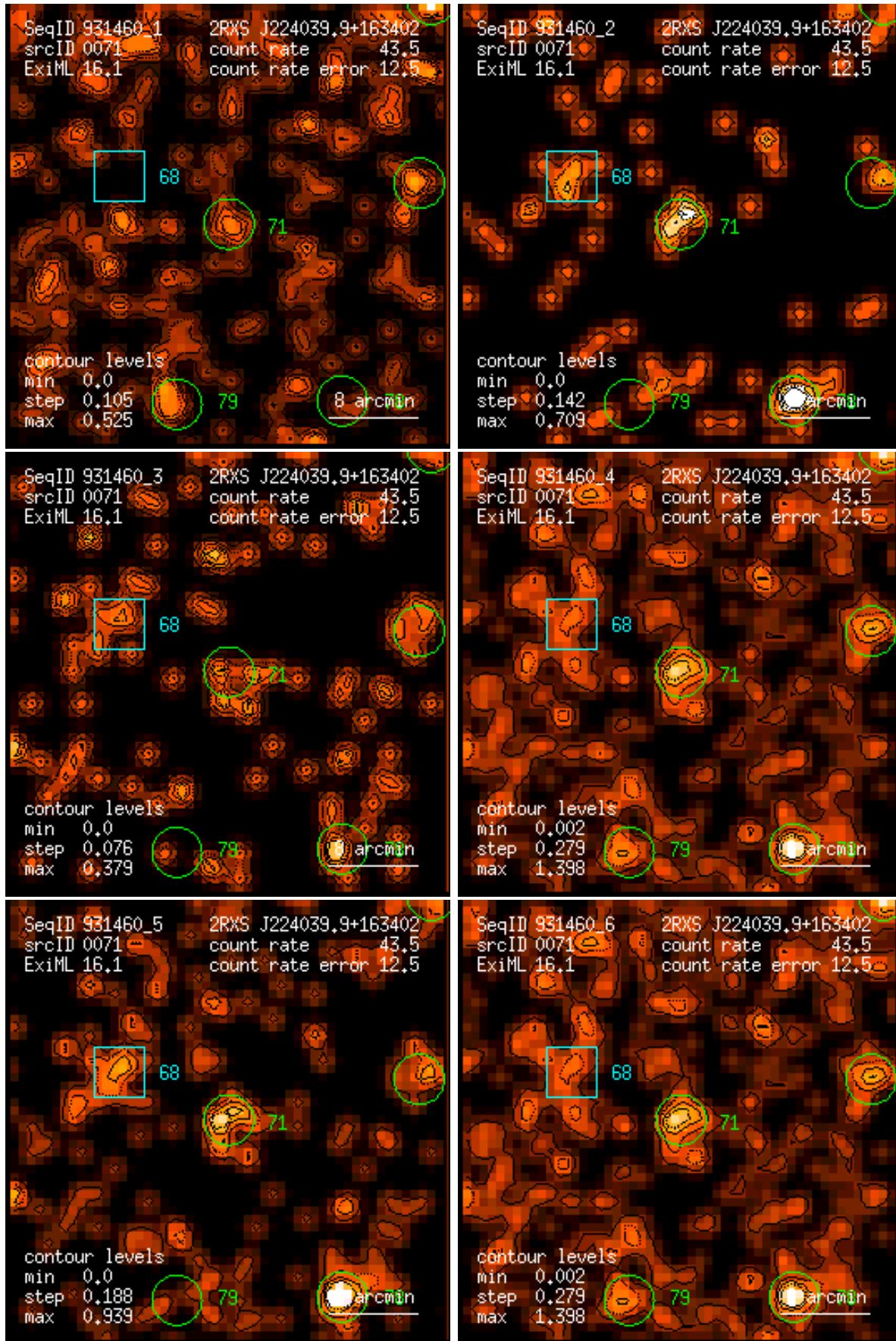
Figure 71: RASS 931460: detection 0071: band rate images, Gaussian filter: (1) PSPC channels 11 – 41, (2) 52 – 90, (3) 91 – 201, (4) 11 – 235, (5) 52 – 201, (6) 11 – 201. Broad band rates in counts/ks. Band rate contour levels in counts/ks/arcmin 2 .
