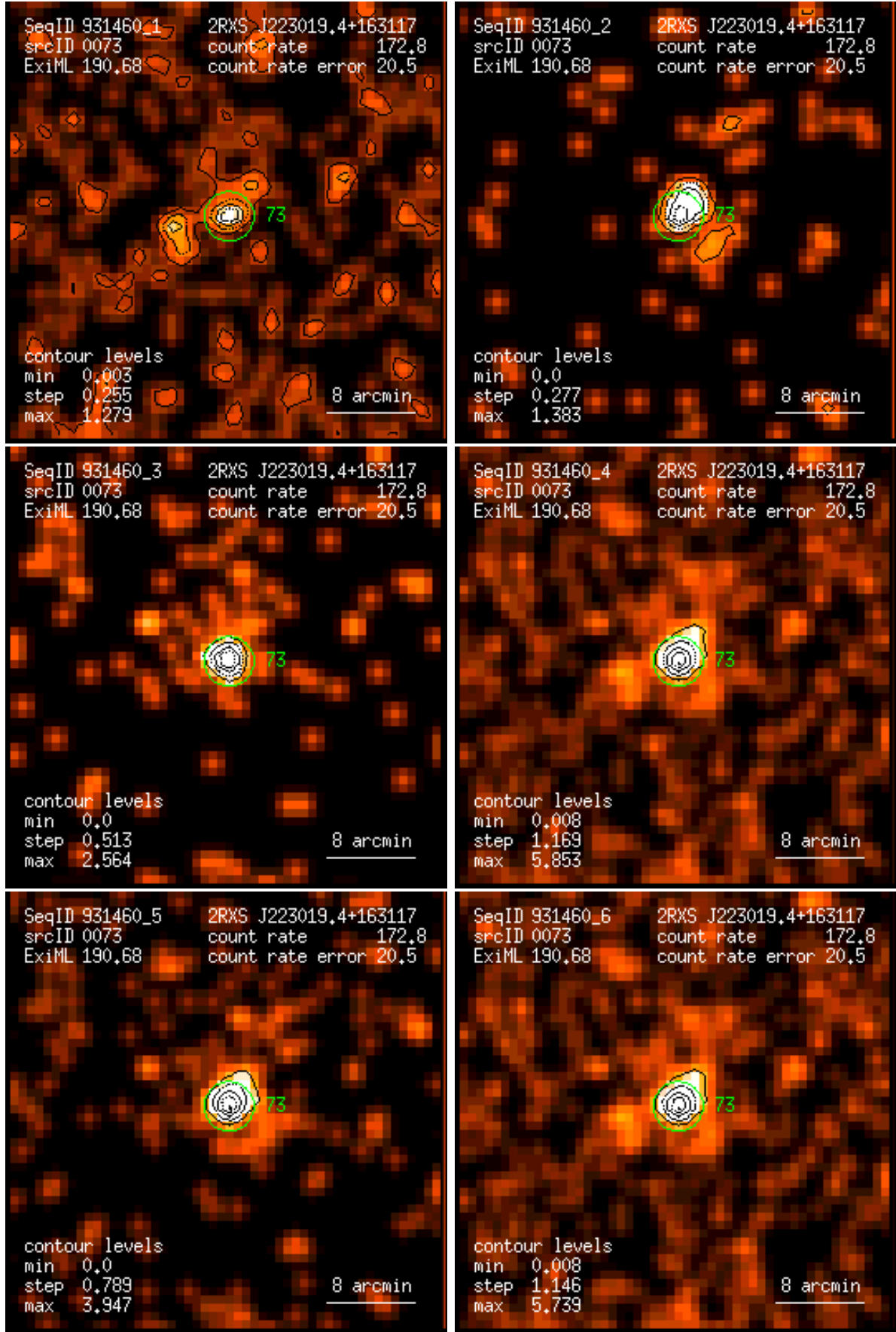
Figure 73: RASS 931460: detection 0073: band rate images, Gaussian filter: (1) PSPC channels 11 – 41, (2) 52 – 90, (3) 91 – 201, (4) 11 – 235, (5) 52 – 201, (6) 11 – 201. Broad band rates in counts/ks. Band rate contour levels in counts/ks/arcmin 2 .
