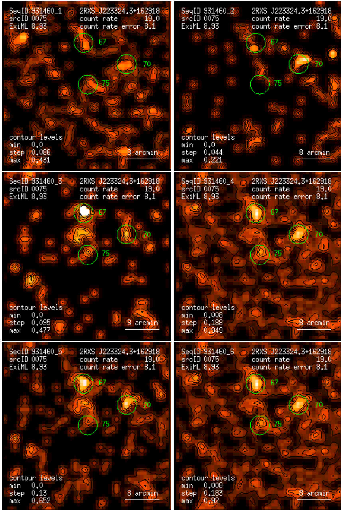
Figure 75: RASS 931460: detection 0075: band rate images, Gaussian filter: (1) PSPC channels 11 – 41, (2) 52 – 90, (3) 91 – 201, (4) 11 – 235, (5) 52 – 201, (6) 11 – 201. Broad band rates in counts/ks. Band rate contour levels in counts/ks/arcmin 2 .
