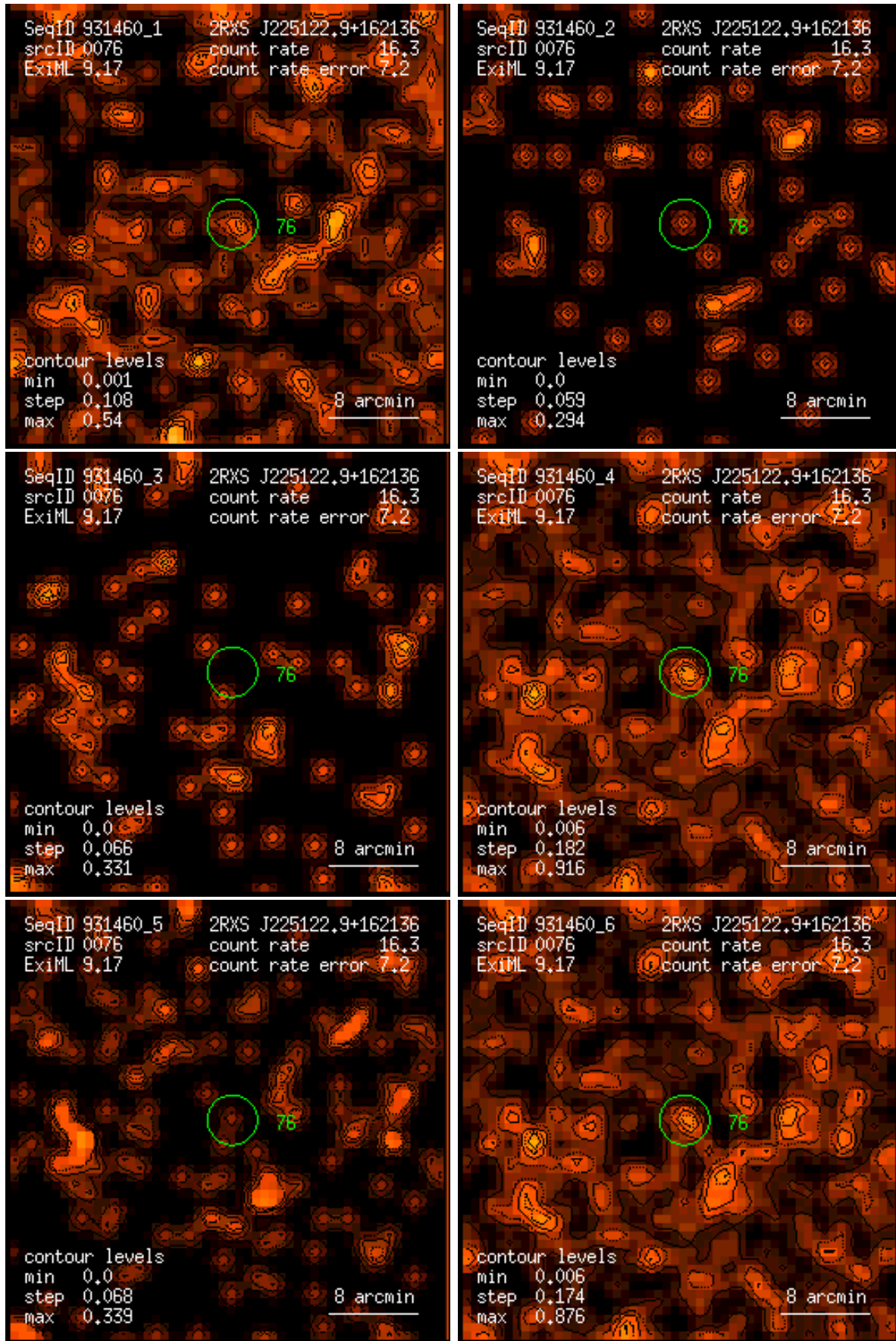
Figure 76: RASS 931460: detection 0076: band rate images, Gaussian filter: (1) PSPC channels 11 – 41, (2) 52 – 90, (3) 91 – 201, (4) 11 – 235, (5) 52 – 201, (6) 11 – 201. Broad band rates in counts/ks. Band rate contour levels in counts/ks/arcmin 2 .
