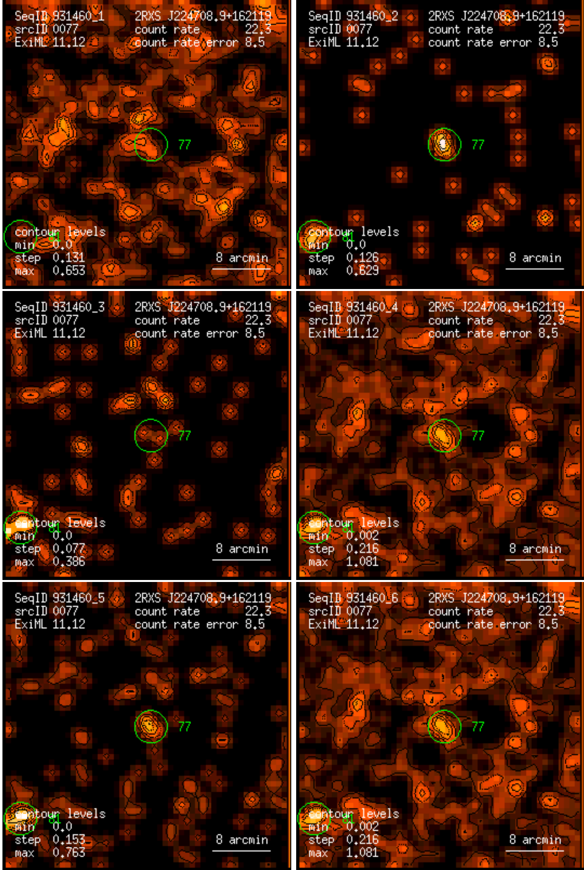
Figure 77: RASS 931460: detection 0077: band rate images, Gaussian filter: (1) PSPC channels 11 – 41, (2) 52 – 90, (3) 91 – 201, (4) 11 – 235, (5) 52 – 201, (6) 11 – 201. Broad band rates in counts/ks. Band rate contour levels in counts/ks/arcmin 2 .
