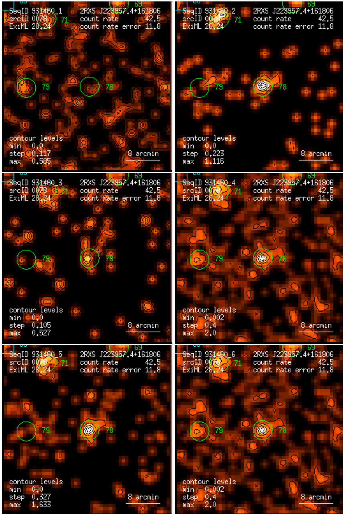
Figure 78: RASS 931460: detection 0078: band rate images, Gaussian filter: (1) PSPC channels 11 – 41, (2) 52 – 90, (3) 91 – 201, (4) 11 – 235, (5) 52 – 201, (6) 11 – 201. Broad band rates in counts/ks. Band rate contour levels in counts/ks/arcmin 2 .
