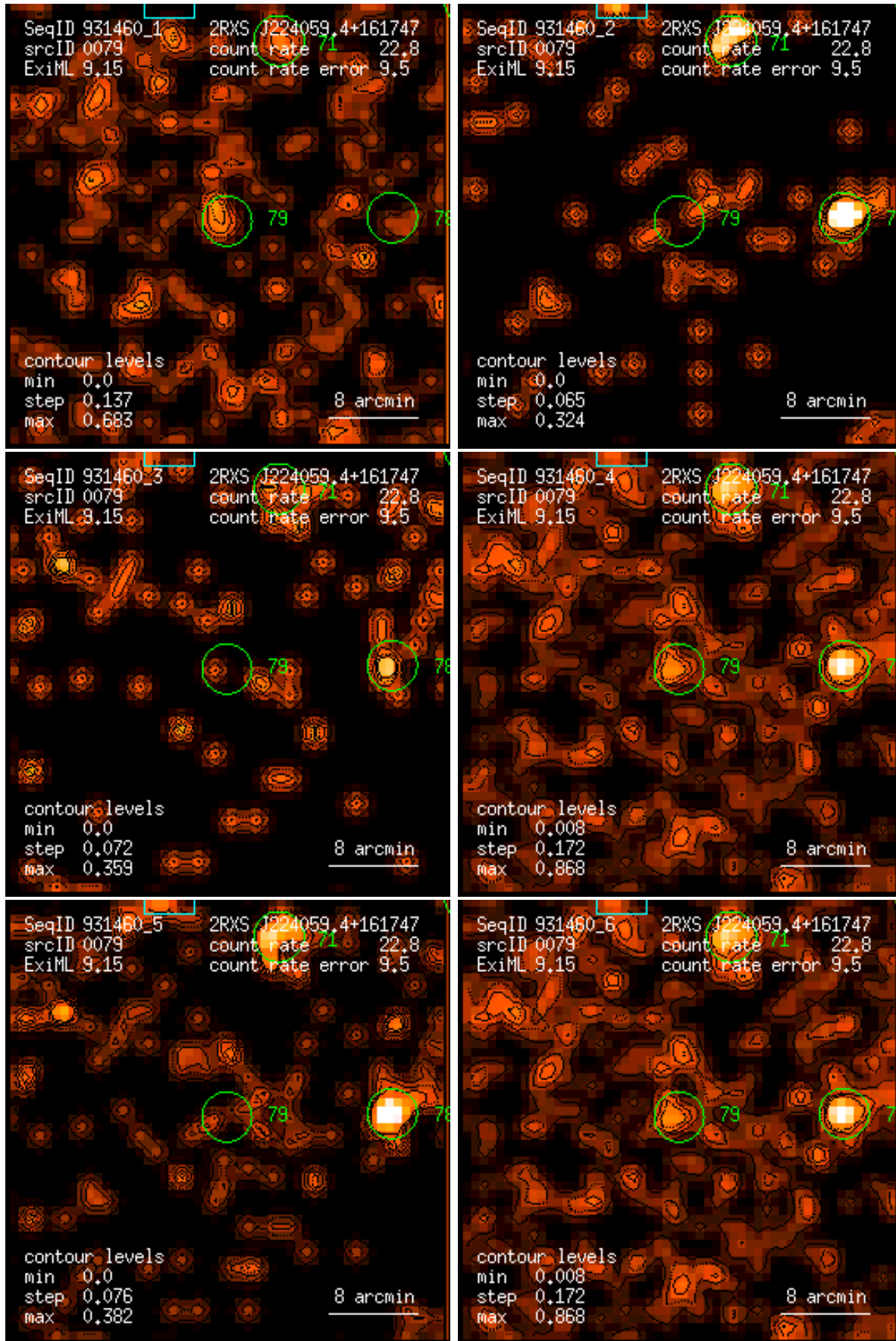
Figure 79: RASS 931460: detection 0079: band rate images, Gaussian filter: (1) PSPC channels 11 – 41, (2) 52 – 90, (3) 91 – 201, (4) 11 – 235, (5) 52 – 201, (6) 11 – 201. Broad band rates in counts/ks. Band rate contour levels in counts/ks/arcmin 2 .
