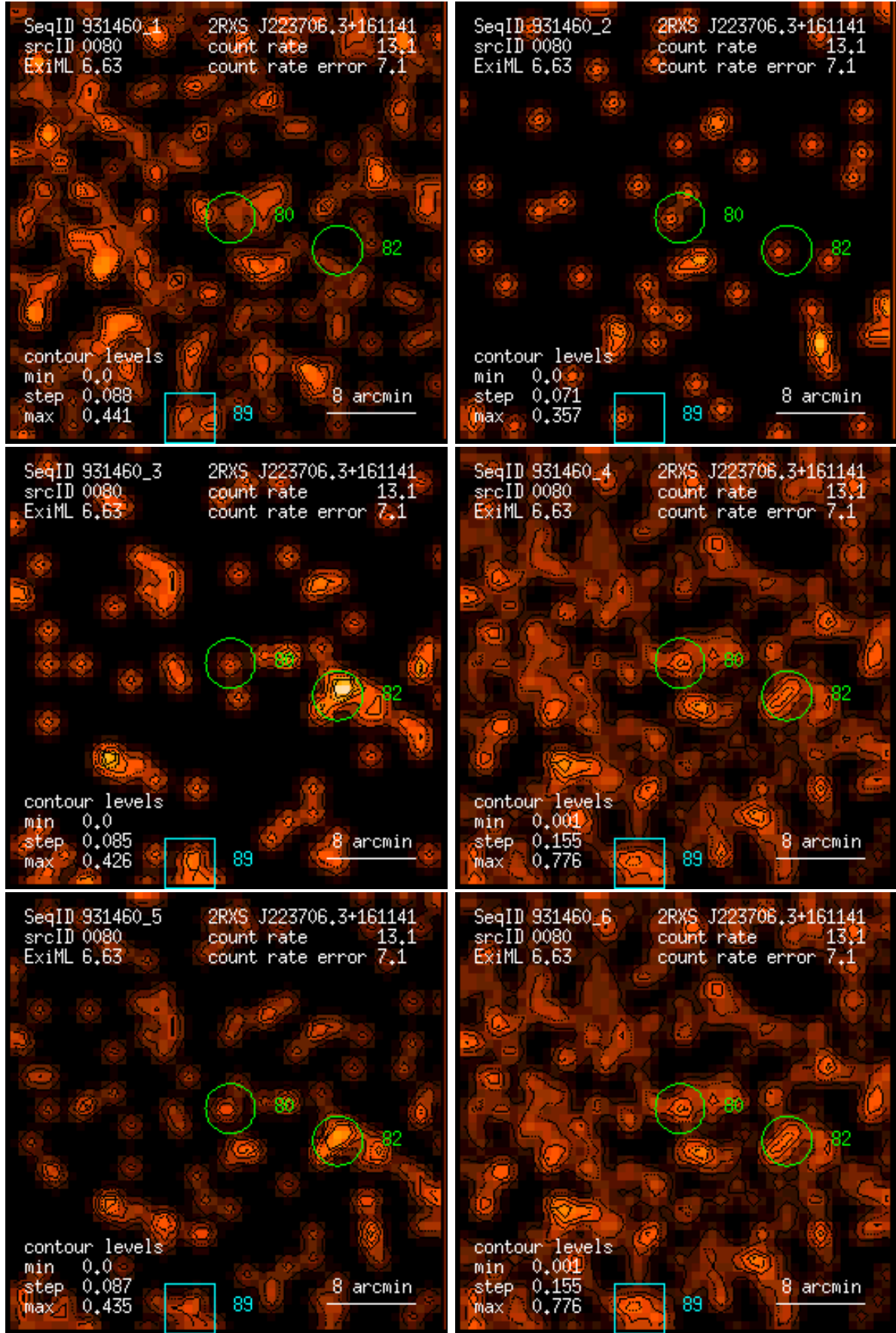
Figure 80: RASS 931460: detection 0080: band rate images, Gaussian filter: (1) PSPC channels 11 – 41, (2) 52 – 90, (3) 91 – 201, (4) 11 – 235, (5) 52 – 201, (6) 11 – 201. Broad band rates in counts/ks. Band rate contour levels in counts/ks/arcmin 2 .
