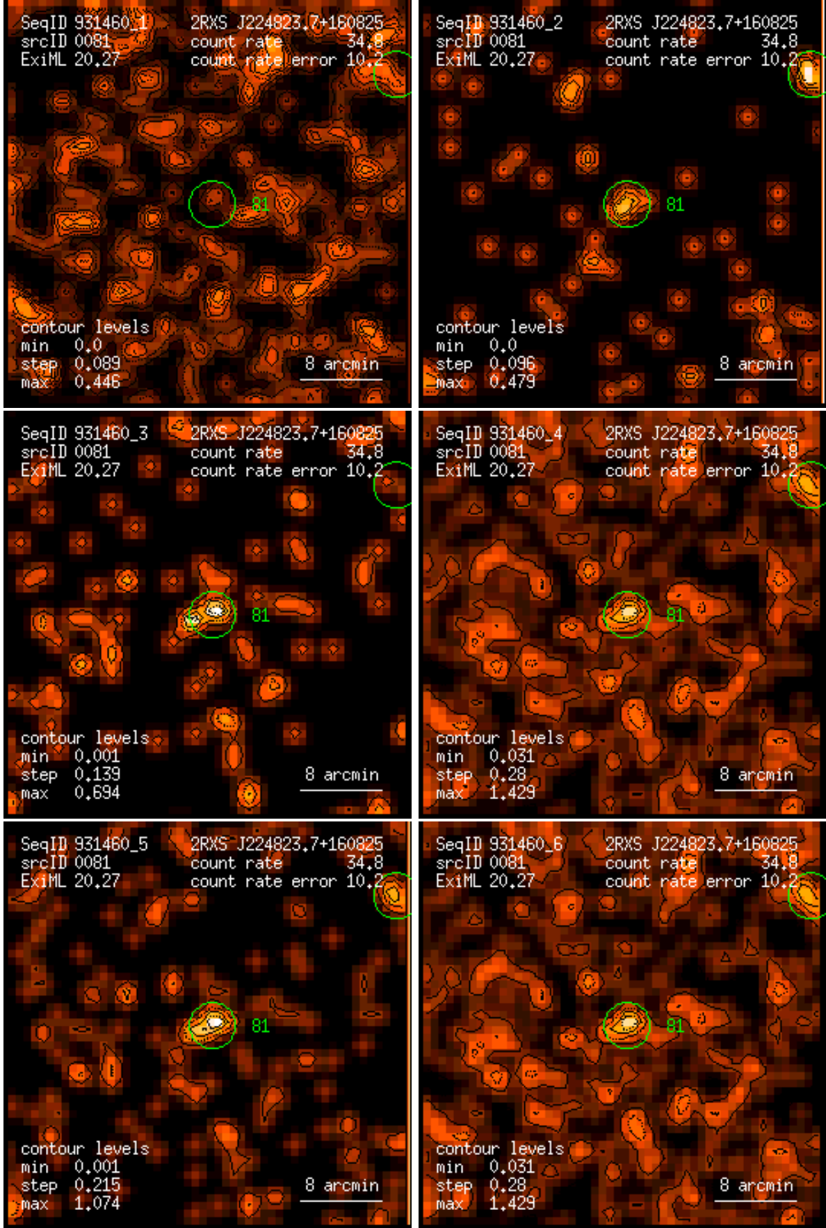
Figure 81: RASS 931460: detection 0081: band rate images, Gaussian filter: (1) PSPC channels 11 – 41, (2) 52 – 90, (3) 91 – 201, (4) 11 – 235, (5) 52 – 201, (6) 11 – 201. Broad band rates in counts/ks. Band rate contour levels in counts/ks/arcmin 2 .
