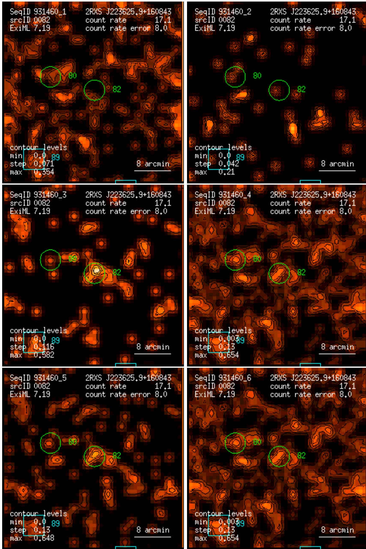
Figure 82: RASS 931460: detection 0082: band rate images, Gaussian filter: (1) PSPC channels 11 – 41, (2) 52 – 90, (3) 91 – 201, (4) 11 – 235, (5) 52 – 201, (6) 11 – 201. Broad band rates in counts/ks. Band rate contour levels in counts/ks/arcmin 2 .
