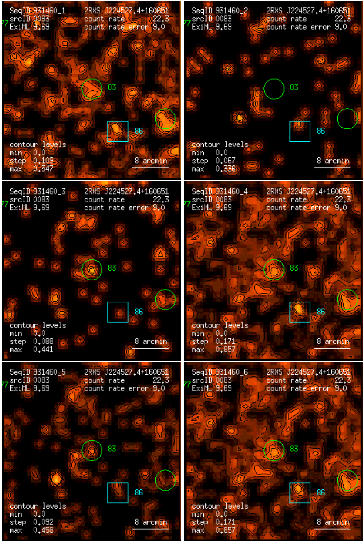
Figure 83: RASS 931460: detection 0083: band rate images, Gaussian filter: (1) PSPC channels 11 – 41, (2) 52 – 90, (3) 91 – 201, (4) 11 – 235, (5) 52 – 201, (6) 11 – 201. Broad band rates in counts/ks. Band rate contour levels in counts/ks/arcmin 2 .
