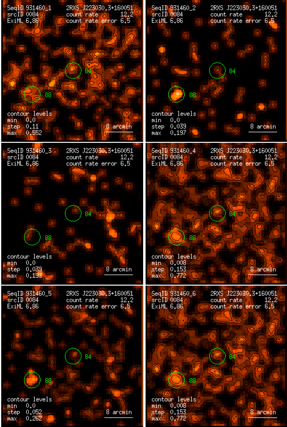
Figure 84: RASS 931460: detection 0084: band rate images, Gaussian filter: (1) PSPC channels 11 – 41, (2) 52 – 90, (3) 91 – 201, (4) 11 – 235, (5) 52 – 201, (6) 11 – 201. Broad band rates in counts/ks. Band rate contour levels in counts/ks/arcmin 2 .
