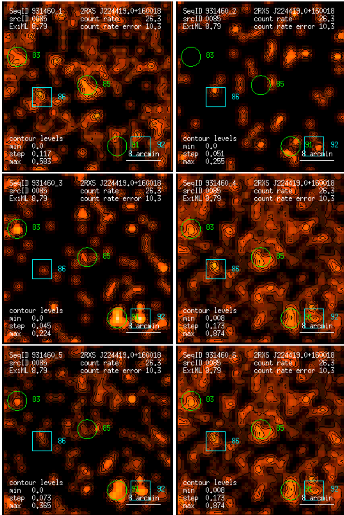
Figure 85: RASS 931460: detection 0085: band rate images, Gaussian filter: (1) PSPC channels 11 – 41, (2) 52 – 90, (3) 91 – 201, (4) 11 – 235, (5) 52 – 201, (6) 11 – 201. Broad band rates in counts/ks. Band rate contour levels in counts/ks/arcmin 2 .
