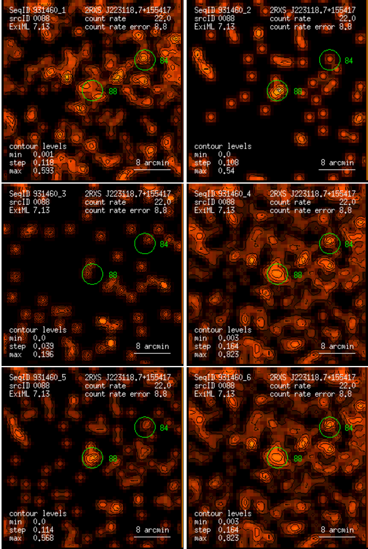
Figure 88: RASS 931460: detection 0088: band rate images, Gaussian filter: (1) PSPC channels 11 – 41, (2) 52 – 90, (3) 91 – 201, (4) 11 – 235, (5) 52 – 201, (6) 11 – 201. Broad band rates in counts/ks. Band rate contour levels in counts/ks/arcmin 2 .
