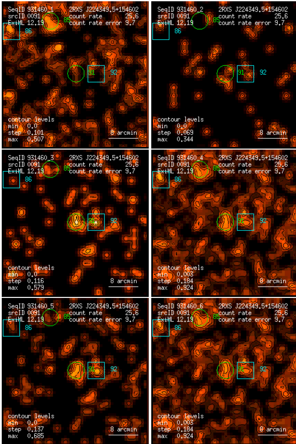
Figure 91: RASS 931460: detection 0091: band rate images, Gaussian filter: (1) PSPC channels 11 – 41, (2) 52 – 90, (3) 91 – 201, (4) 11 – 235, (5) 52 – 201, (6) 11 – 201. Broad band rates in counts/ks. Band rate contour levels in counts/ks/arcmin 2 .
