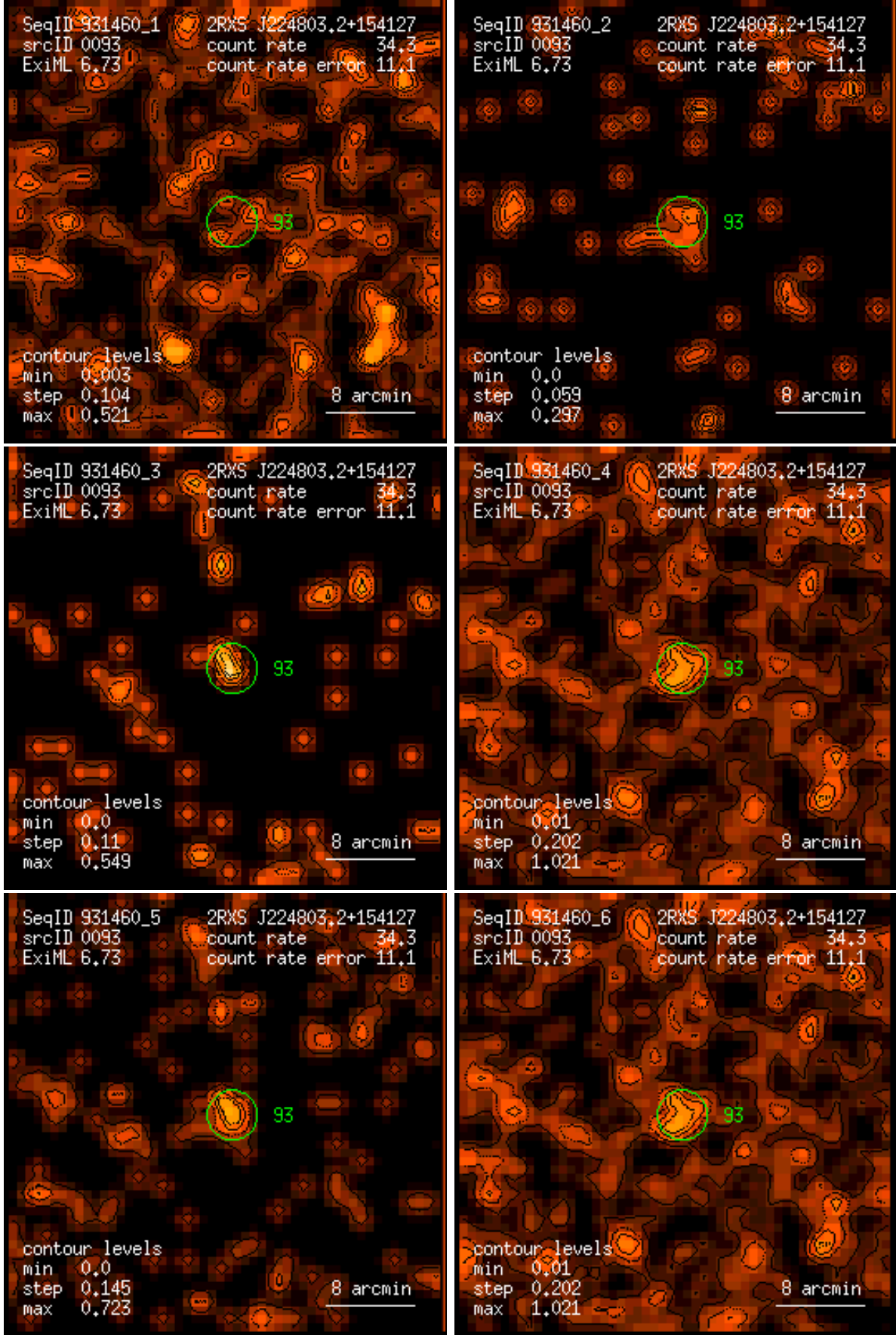
Figure 93: RASS 931460: detection 0093: band rate images, Gaussian filter: (1) PSPC channels 11 – 41, (2) 52 – 90, (3) 91 – 201, (4) 11 – 235, (5) 52 – 201, (6) 11 – 201. Broad band rates in counts/ks. Band rate contour levels in counts/ks/arcmin 2 .
