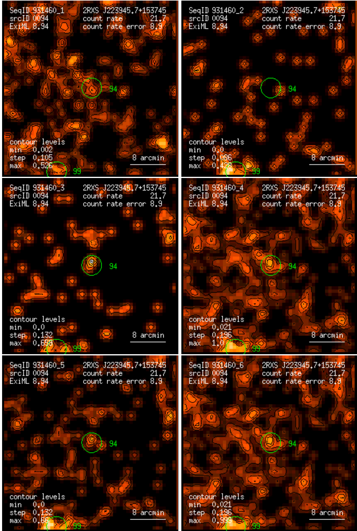
Figure 94: RASS 931460: detection 0094: band rate images, Gaussian filter: (1) PSPC channels 11 – 41, (2) 52 – 90, (3) 91 – 201, (4) 11 – 235, (5) 52 – 201, (6) 11 – 201. Broad band rates in counts/ks. Band rate contour levels in counts/ks/arcmin 2 .
