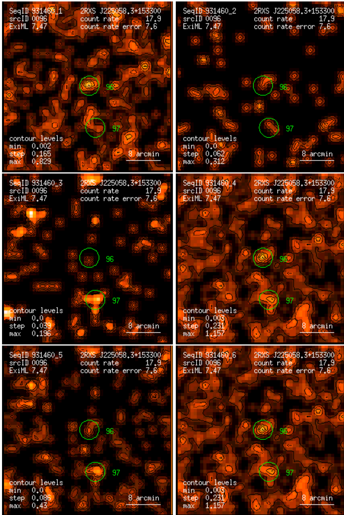
Figure 96: RASS 931460: detection 0096: band rate images, Gaussian filter: (1) PSPC channels 11 – 41, (2) 52 – 90, (3) 91 – 201, (4) 11 – 235, (5) 52 – 201, (6) 11 – 201. Broad band rates in counts/ks. Band rate contour levels in counts/ks/arcmin 2 .
