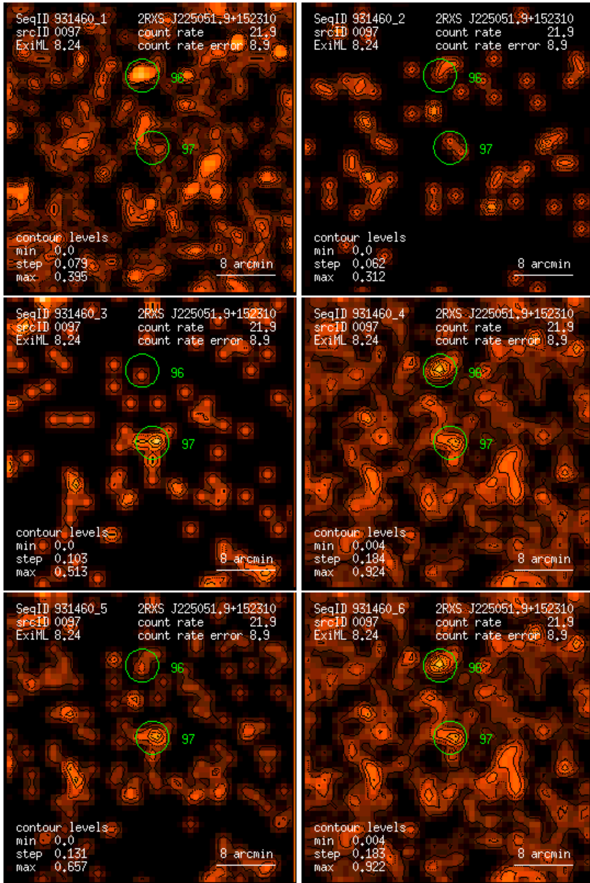
Figure 97: RASS 931460: detection 0097: band rate images, Gaussian filter: (1) PSPC channels 11 – 41, (2) 52 – 90, (3) 91 – 201, (4) 11 – 235, (5) 52 – 201, (6) 11 – 201. Broad band rates in counts/ks. Band rate contour levels in counts/ks/arcmin 2 .
