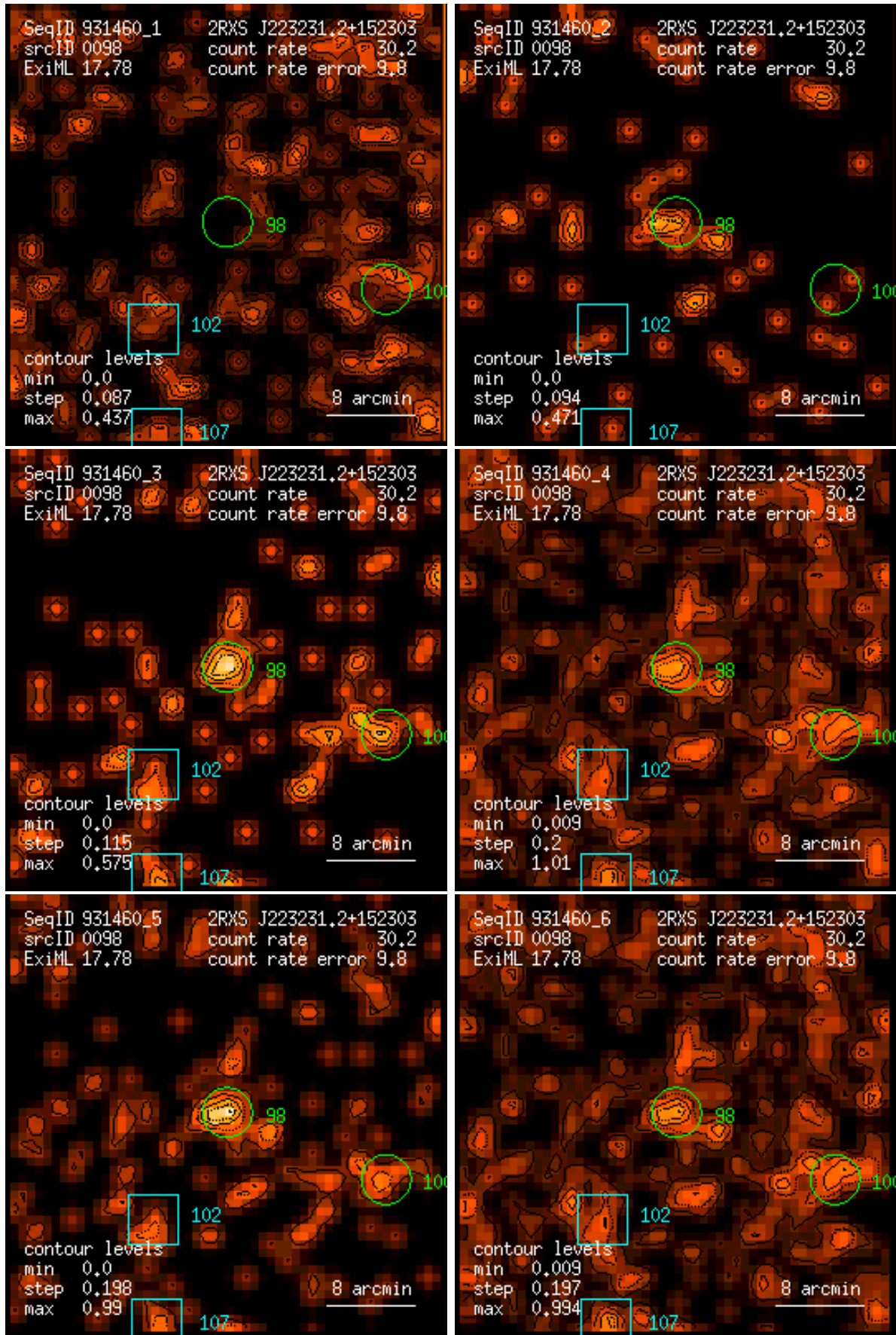
Figure 98: RASS 931460: detection 0098: band rate images, Gaussian filter: (1) PSPC channels 11 – 41, (2) 52 – 90, (3) 91 – 201, (4) 11 – 235, (5) 52 – 201, (6) 11 – 201. Broad band rates in counts/ks. Band rate contour levels in counts/ks/arcmin 2 .
