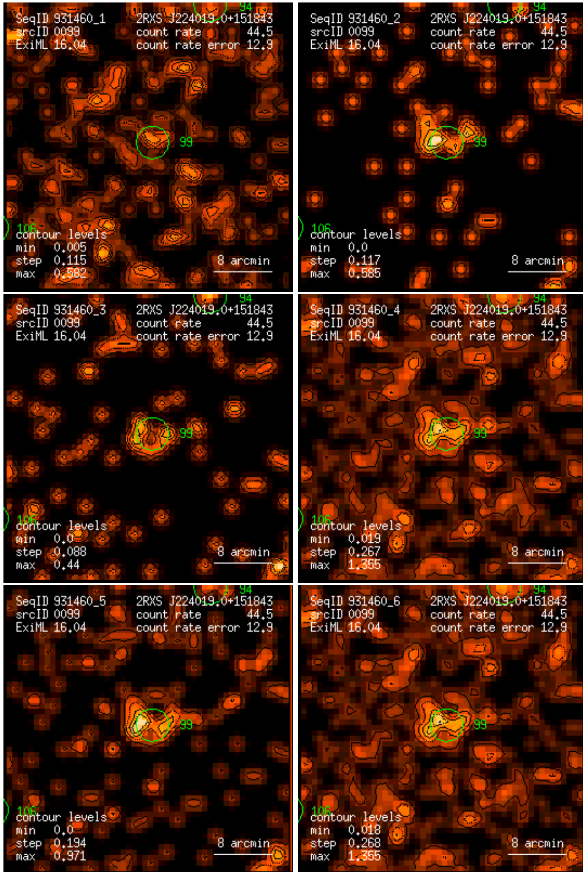
Figure 99: RASS 931460: detection 0099: band rate images, Gaussian filter: (1) PSPC channels 11 – 41, (2) 52 – 90, (3) 91 – 201, (4) 11 – 235, (5) 52 – 201, (6) 11 – 201. Broad band rates in counts/ks. Band rate contour levels in counts/ks/arcmin 2 .
