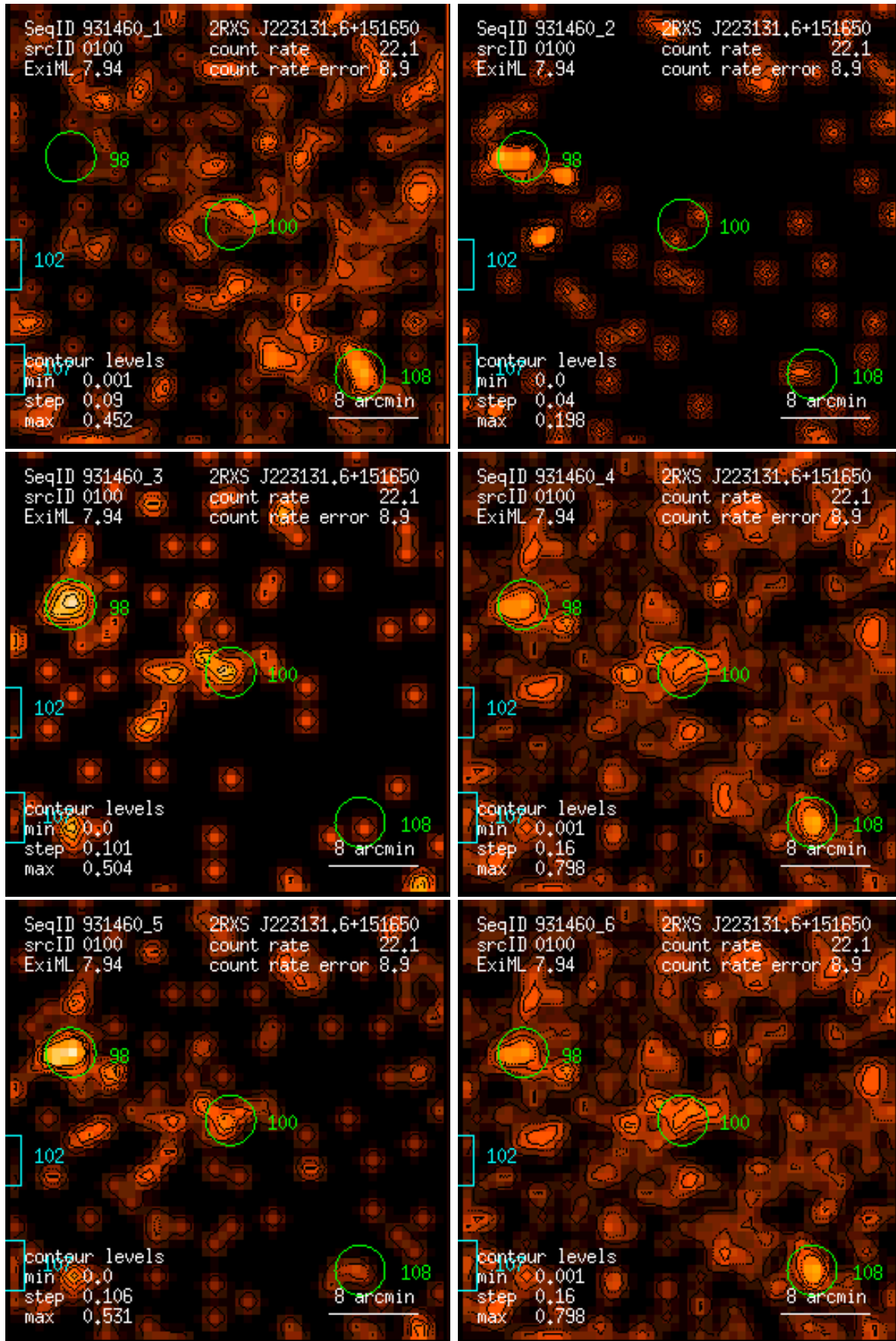
Figure 100: RASS 931460: detection 0100: band rate images, Gaussian filter: (1) PSPC channels 11 – 41, (2) 52 – 90, (3) 91 – 201, (4) 11 – 235, (5) 52 – 201, (6) 11 – 201. Broad band rates in counts/ks. Band rate contour levels in counts/ks/arcmin 2 .
